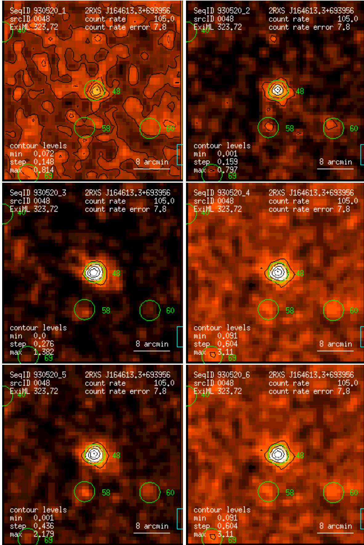
Figure 48: RASS 930520: detection 0048: band rate images, Gaussian filter: (1) PSPC channels 11 – 41, (2) 52 – 90, (3) 91 – 201, (4) 11 – 235, (5) 52 – 201, (6) 11 – 201. Broad band rates in counts/ks. Band rate contour levels in counts/ks/arcmin 2 .
