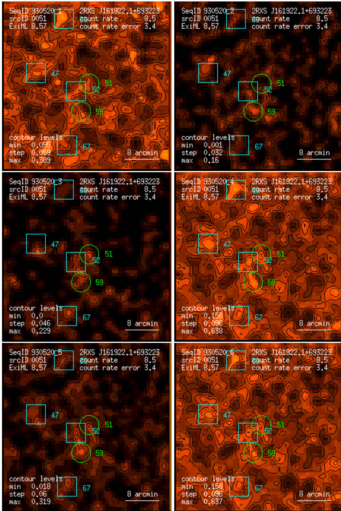
Figure 51: RASS 930520: detection 0051: band rate images, Gaussian filter: (1) PSPC channels 11 – 41, (2) 52 – 90, (3) 91 – 201, (4) 11 – 235, (5) 52 – 201, (6) 11 – 201. Broad band rates in counts/ks. Band rate contour levels in counts/ks/arcmin 2 .
