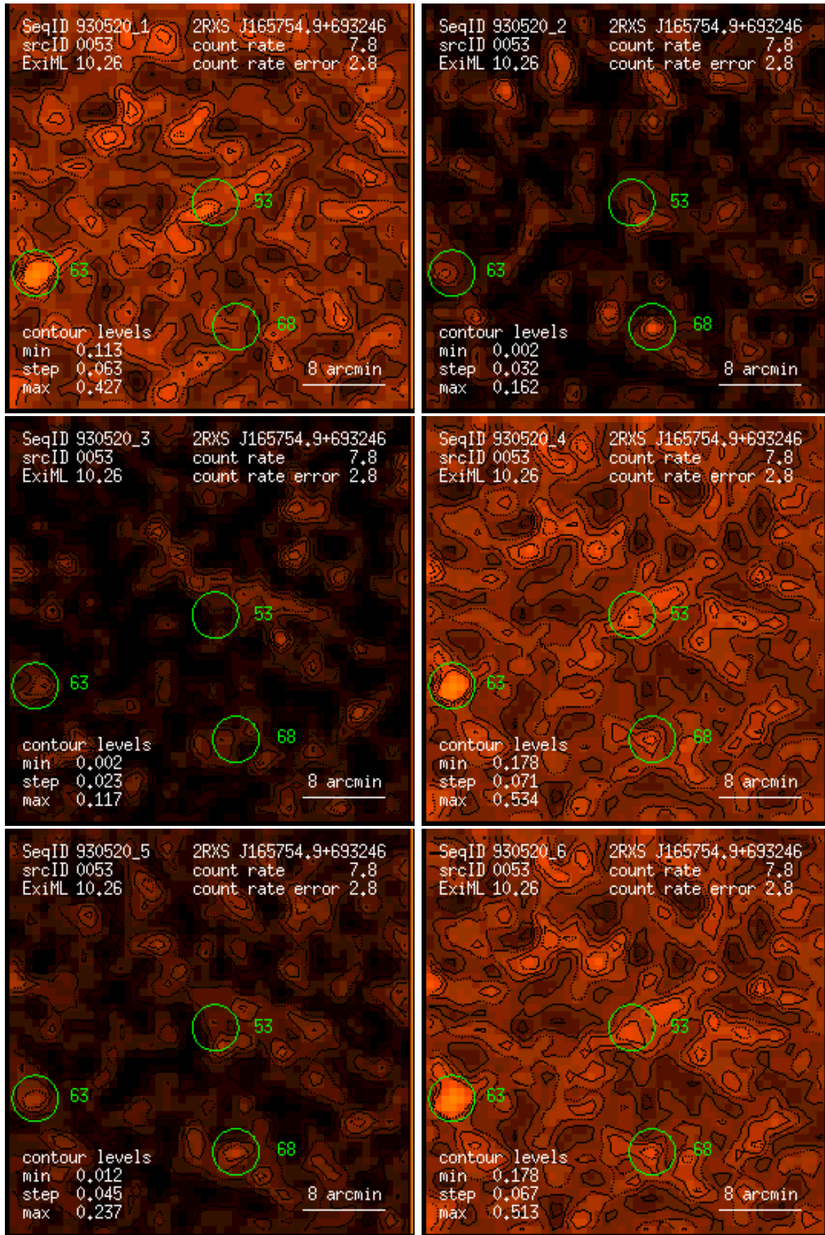
Figure 53: RASS 930520: detection 0053: band rate images, Gaussian filter: (1) PSPC channels 11 – 41, (2) 52 – 90, (3) 91 – 201, (4) 11 – 235, (5) 52 – 201, (6) 11 – 201. Broad band rates in counts/ks. Band rate contour levels in counts/ks/arcmin 2 .
