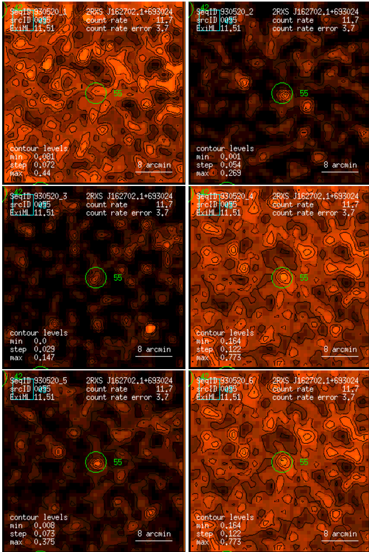
Figure 55: RASS 930520: detection 0055: band rate images, Gaussian filter: (1) PSPC channels 11 – 41, (2) 52 – 90, (3) 91 – 201, (4) 11 – 235, (5) 52 – 201, (6) 11 – 201. Broad band rates in counts/ks. Band rate contour levels in counts/ks/arcmin 2 .
