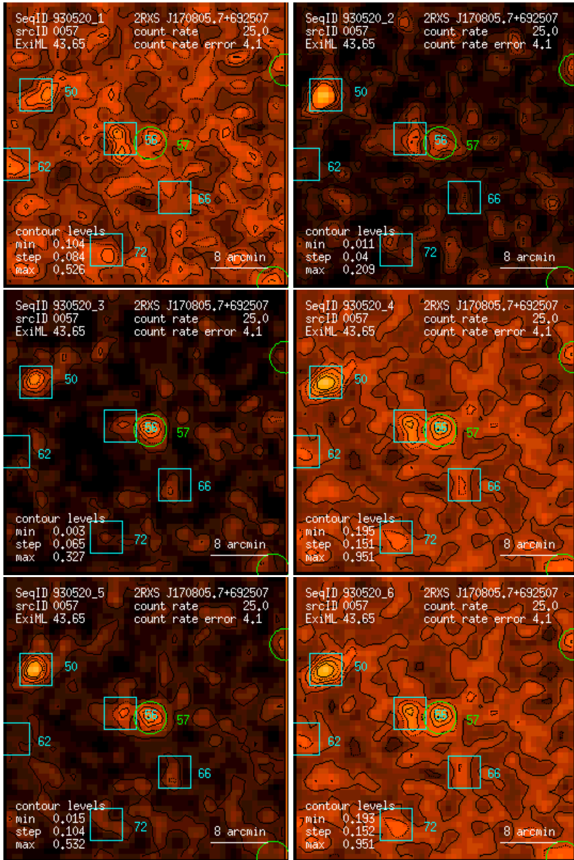
Figure 57: RASS 930520: detection 0057: band rate images, Gaussian filter: (1) PSPC channels 11 – 41, (2) 52 – 90, (3) 91 – 201, (4) 11 – 235, (5) 52 – 201, (6) 11 – 201. Broad band rates in counts/ks. Band rate contour levels in counts/ks/arcmin 2 .
