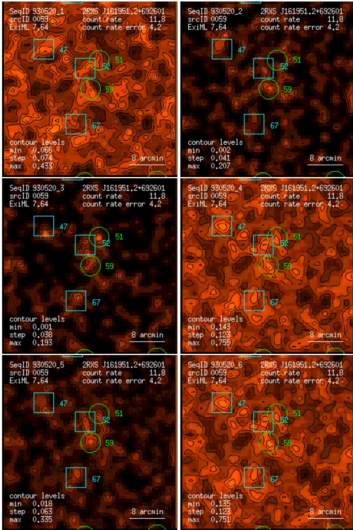
Figure 59: RASS 930520: detection 0059: band rate images, Gaussian filter: (1) PSPC channels 11 – 41, (2) 52 – 90, (3) 91 – 201, (4) 11 – 235, (5) 52 – 201, (6) 11 – 201. Broad band rates in counts/ks. Band rate contour levels in counts/ks/arcmin 2 .
