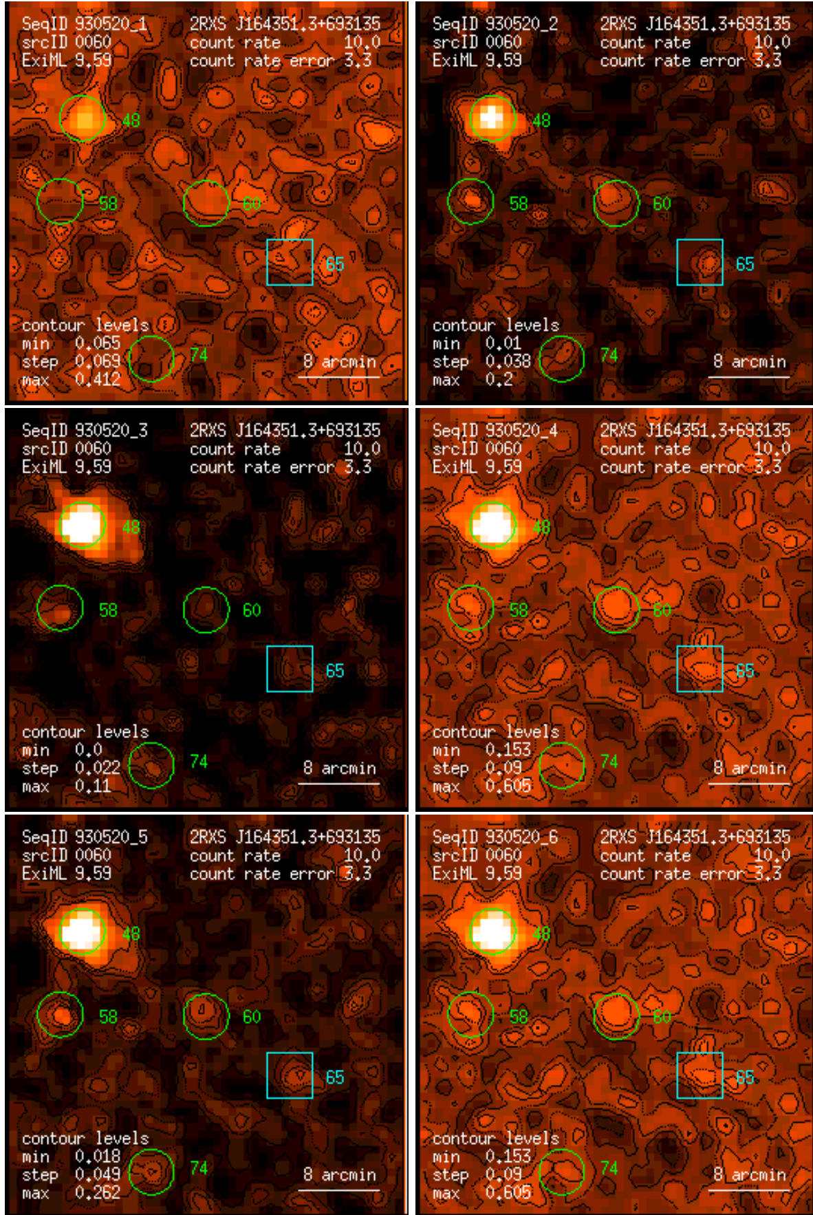
Figure 60: RASS 930520: detection 0060: band rate images, Gaussian filter: (1) PSPC channels 11 – 41, (2) 52 – 90, (3) 91 – 201, (4) 11 – 235, (5) 52 – 201, (6) 11 – 201. Broad band rates in counts/ks. Band rate contour levels in counts/ks/arcmin 2 .
