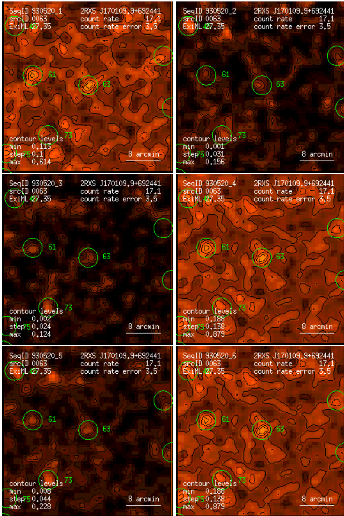
Figure 63: RASS 930520: detection 0063: band rate images, Gaussian filter: (1) PSPC channels 11 – 41, (2) 52 – 90, (3) 91 – 201, (4) 11 – 235, (5) 52 – 201, (6) 11 – 201. Broad band rates in counts/ks. Band rate contour levels in counts/ks/arcmin 2 .
