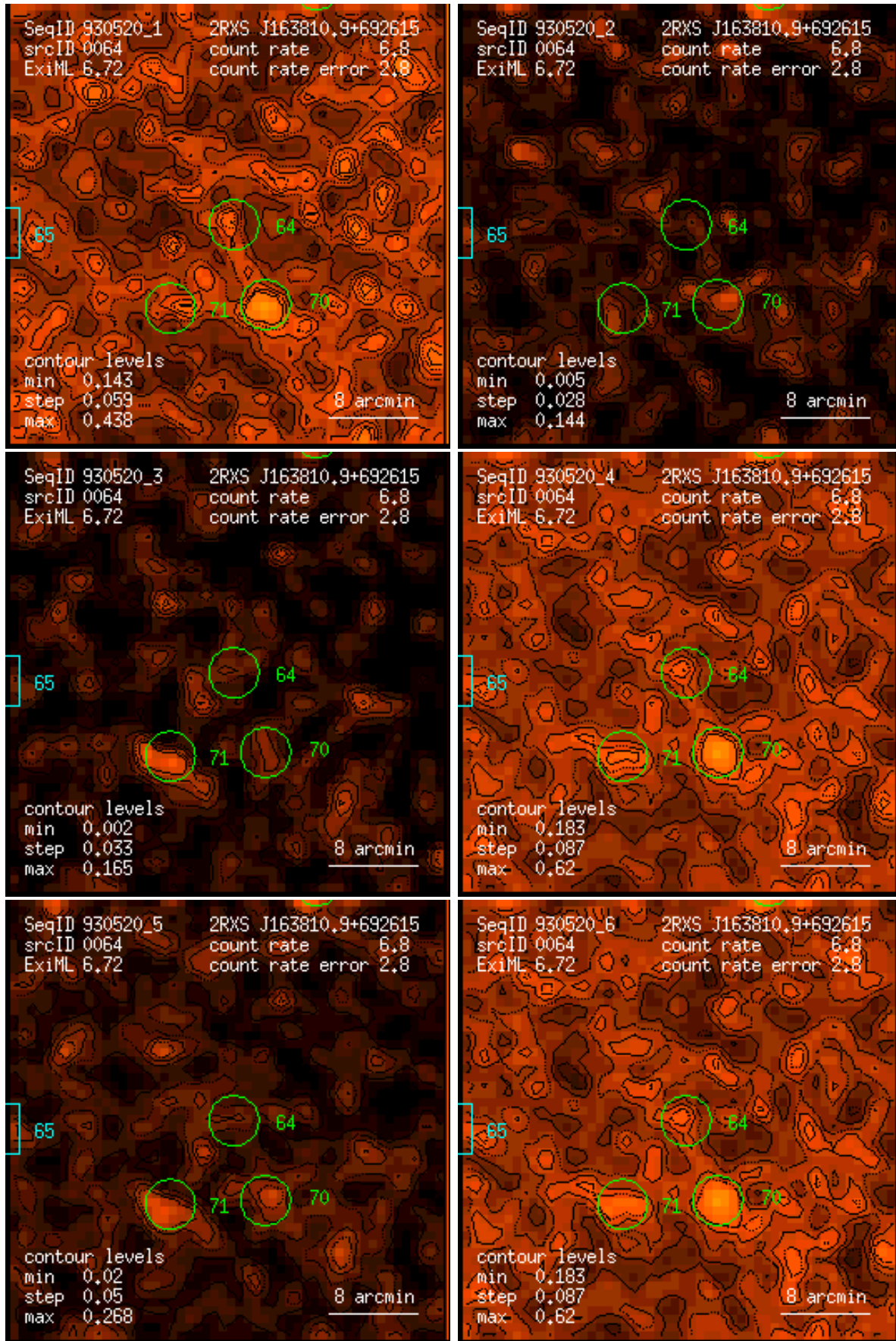
Figure 64: RASS 930520: detection 0064: band rate images, Gaussian filter: (1) PSPC channels 11 – 41, (2) 52 – 90, (3) 91 – 201, (4) 11 – 235, (5) 52 – 201, (6) 11 – 201. Broad band rates in counts/ks. Band rate contour levels in counts/ks/arcmin 2 .
