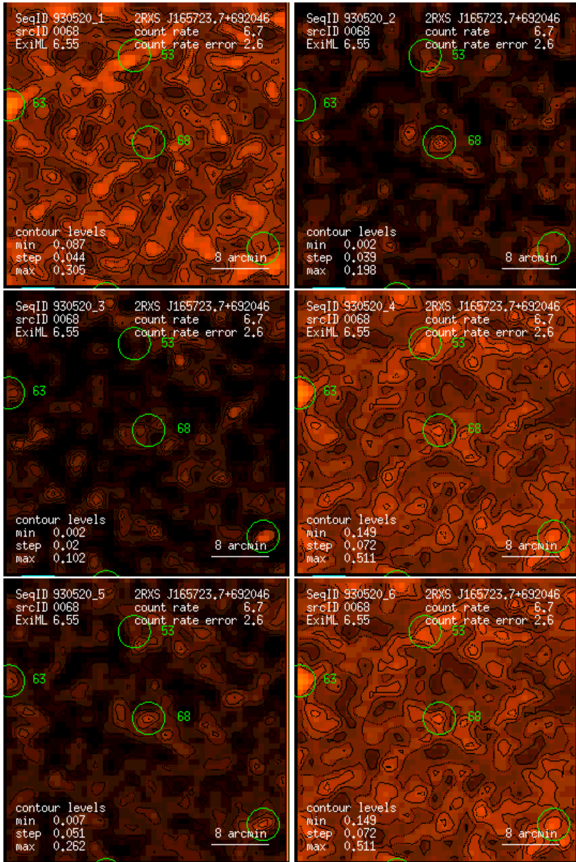
Figure 68: RASS 930520: detection 0068: band rate images, Gaussian filter: (1) PSPC channels 11 – 41, (2) 52 – 90, (3) 91 – 201, (4) 11 – 235, (5) 52 – 201, (6) 11 – 201. Broad band rates in counts/ks. Band rate contour levels in counts/ks/arcmin 2 .
