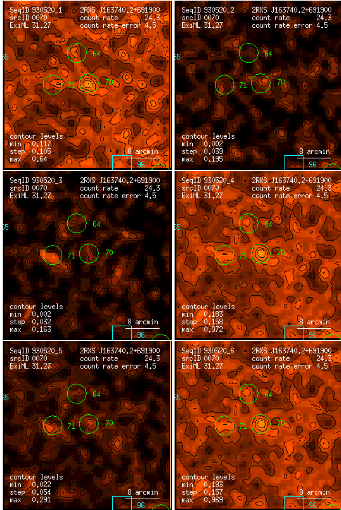
Figure 70: RASS 930520: detection 0070: band rate images, Gaussian filter: (1) PSPC channels 11 – 41, (2) 52 – 90, (3) 91 – 201, (4) 11 – 235, (5) 52 – 201, (6) 11 – 201. Broad band rates in counts/ks. Band rate contour levels in counts/ks/arcmin 2 .
