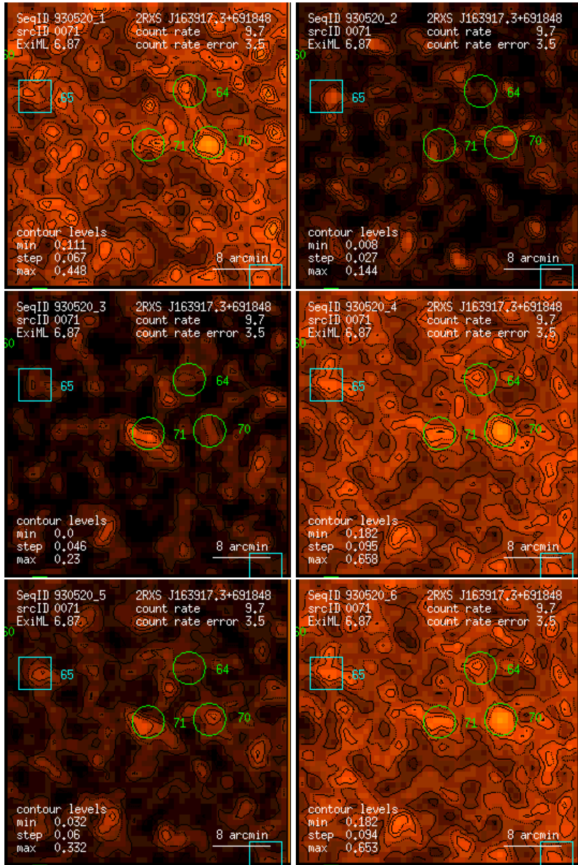
Figure 71: RASS 930520: detection 0071: band rate images, Gaussian filter: (1) PSPC channels 11 – 41, (2) 52 – 90, (3) 91 – 201, (4) 11 – 235, (5) 52 – 201, (6) 11 – 201. Broad band rates in counts/ks. Band rate contour levels in counts/ks/arcmin 2 .
