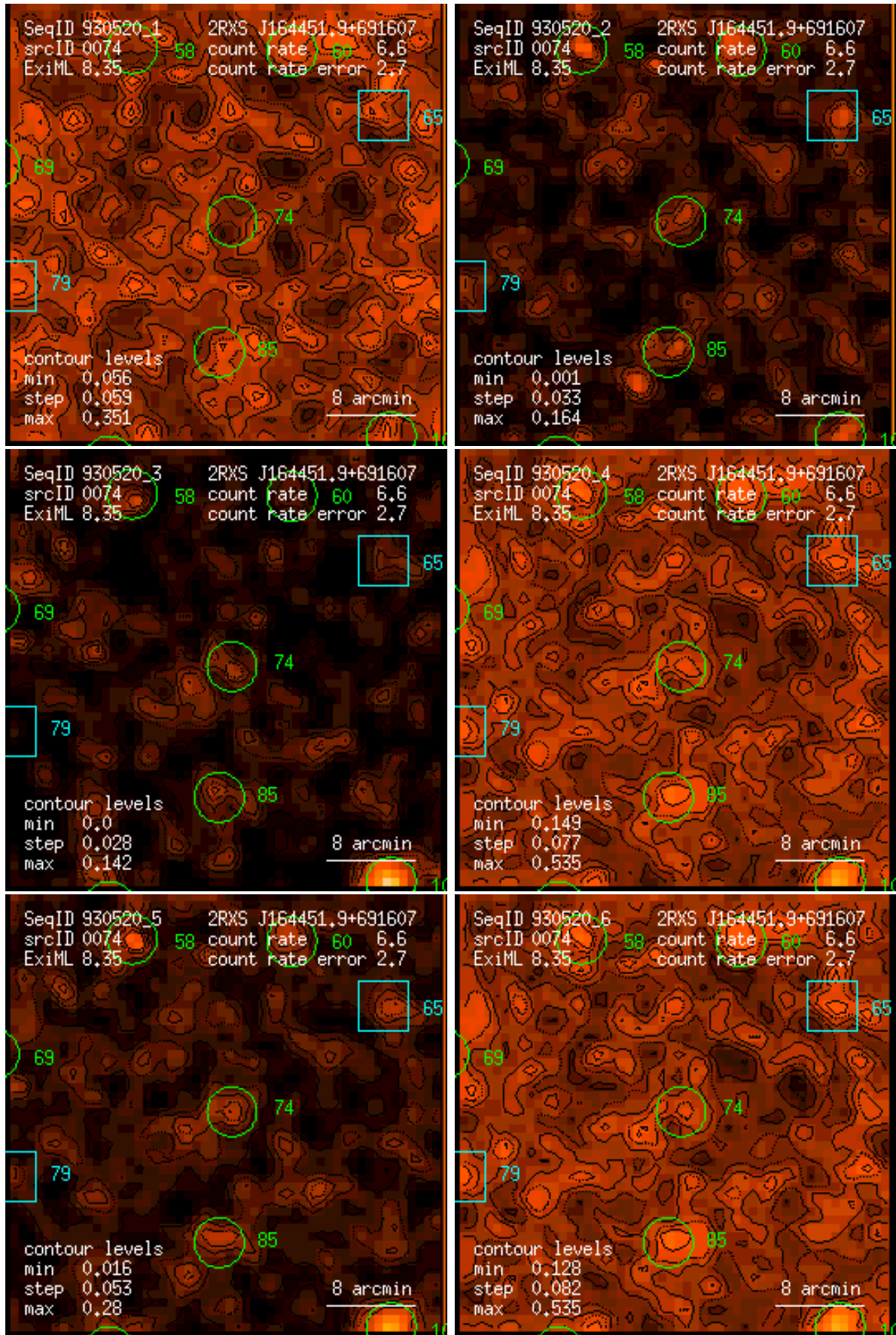
Figure 74: RASS 930520: detection 0074: band rate images, Gaussian filter: (1) PSPC channels 11 – 41, (2) 52 – 90, (3) 91 – 201, (4) 11 – 235, (5) 52 – 201, (6) 11 – 201. Broad band rates in counts/ks. Band rate contour levels in counts/ks/arcmin 2 .
