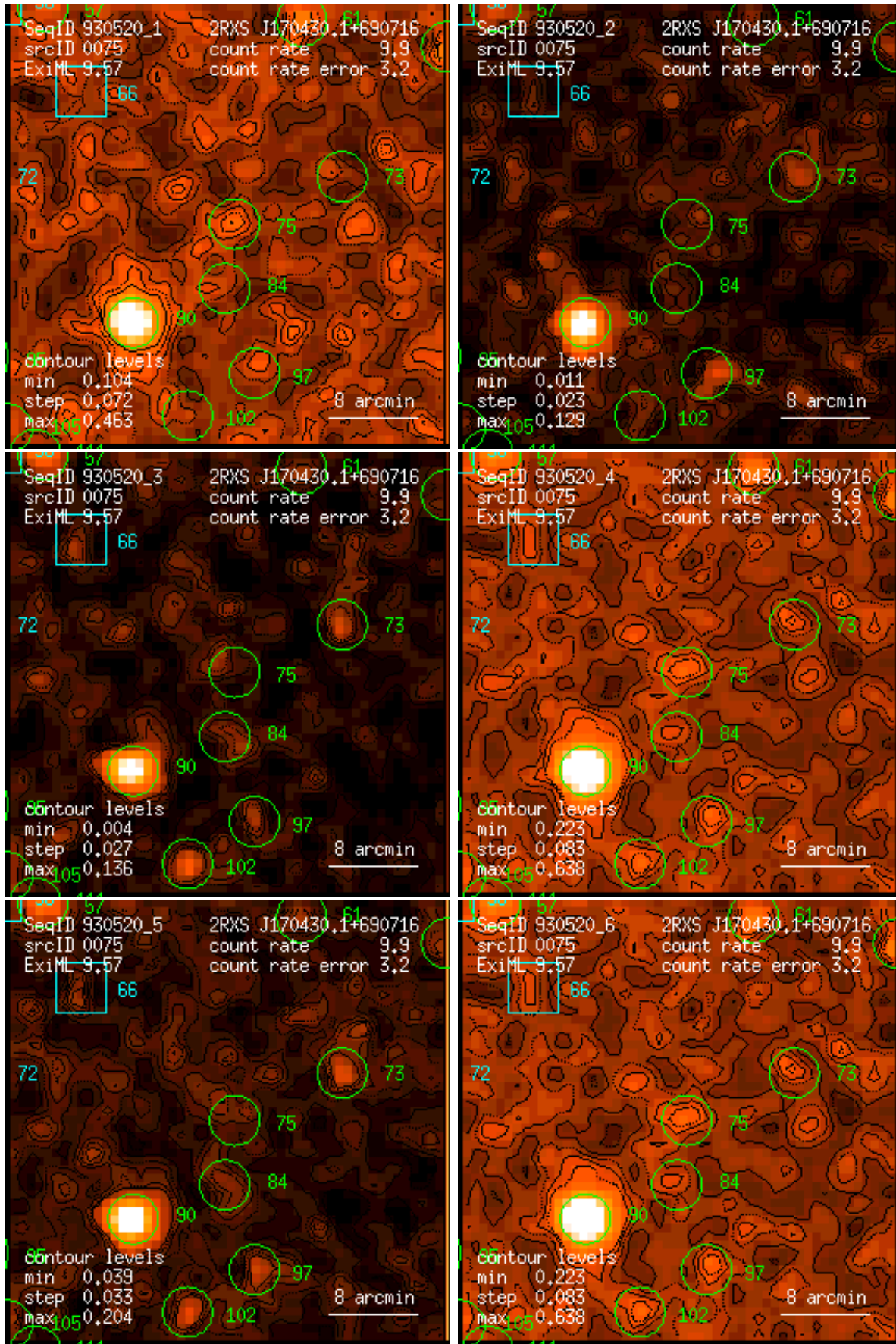
Figure 75: RASS 930520: detection 0075: band rate images, Gaussian filter: (1) PSPC channels 11 – 41, (2) 52 – 90, (3) 91 – 201, (4) 11 – 235, (5) 52 – 201, (6) 11 – 201. Broad band rates in counts/ks. Band rate contour levels in counts/ks/arcmin 2 .
