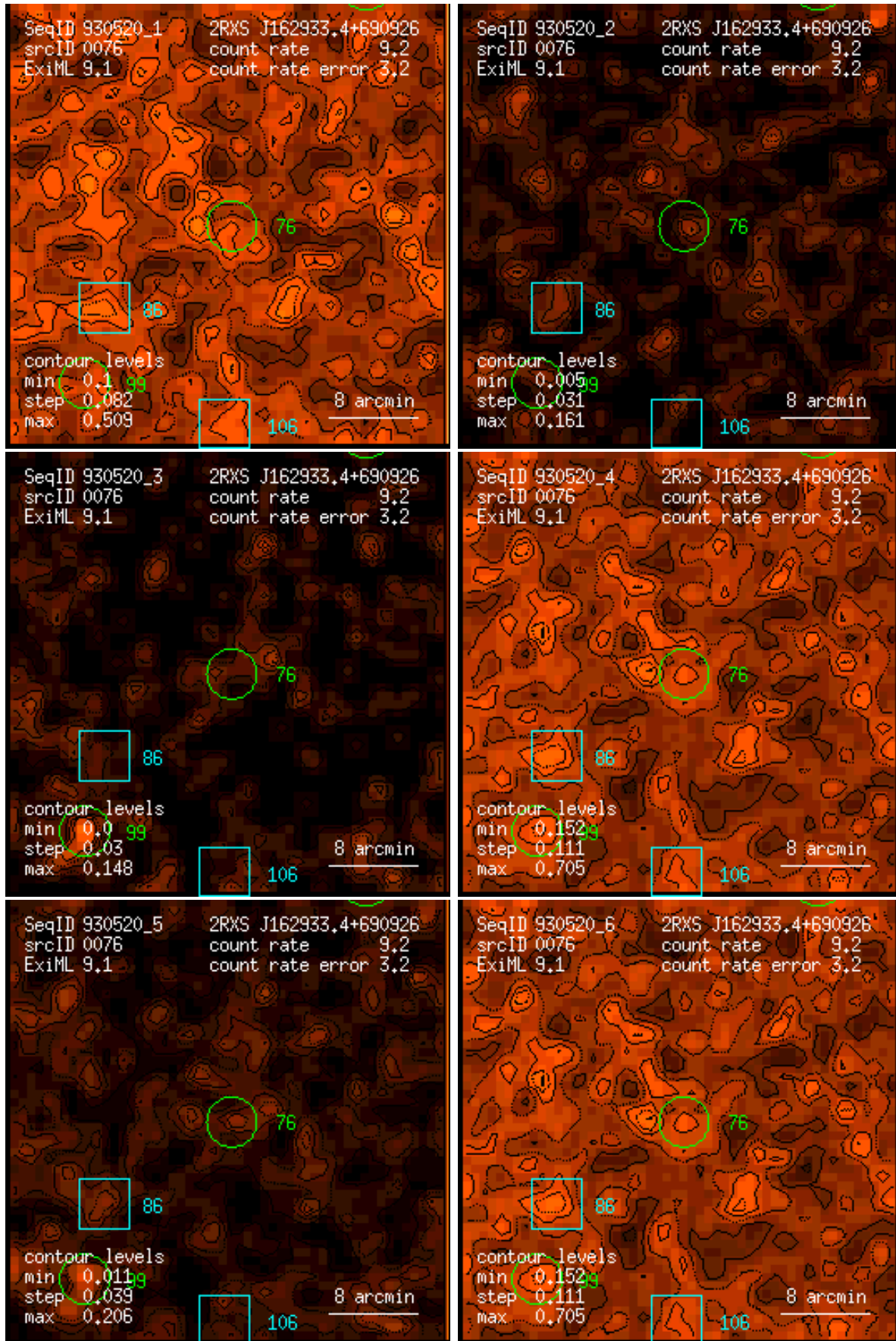
Figure 76: RASS 930520: detection 0076: band rate images, Gaussian filter: (1) PSPC channels 11 – 41, (2) 52 – 90, (3) 91 – 201, (4) 11 – 235, (5) 52 – 201, (6) 11 – 201. Broad band rates in counts/ks. Band rate contour levels in counts/ks/arcmin 2 .
