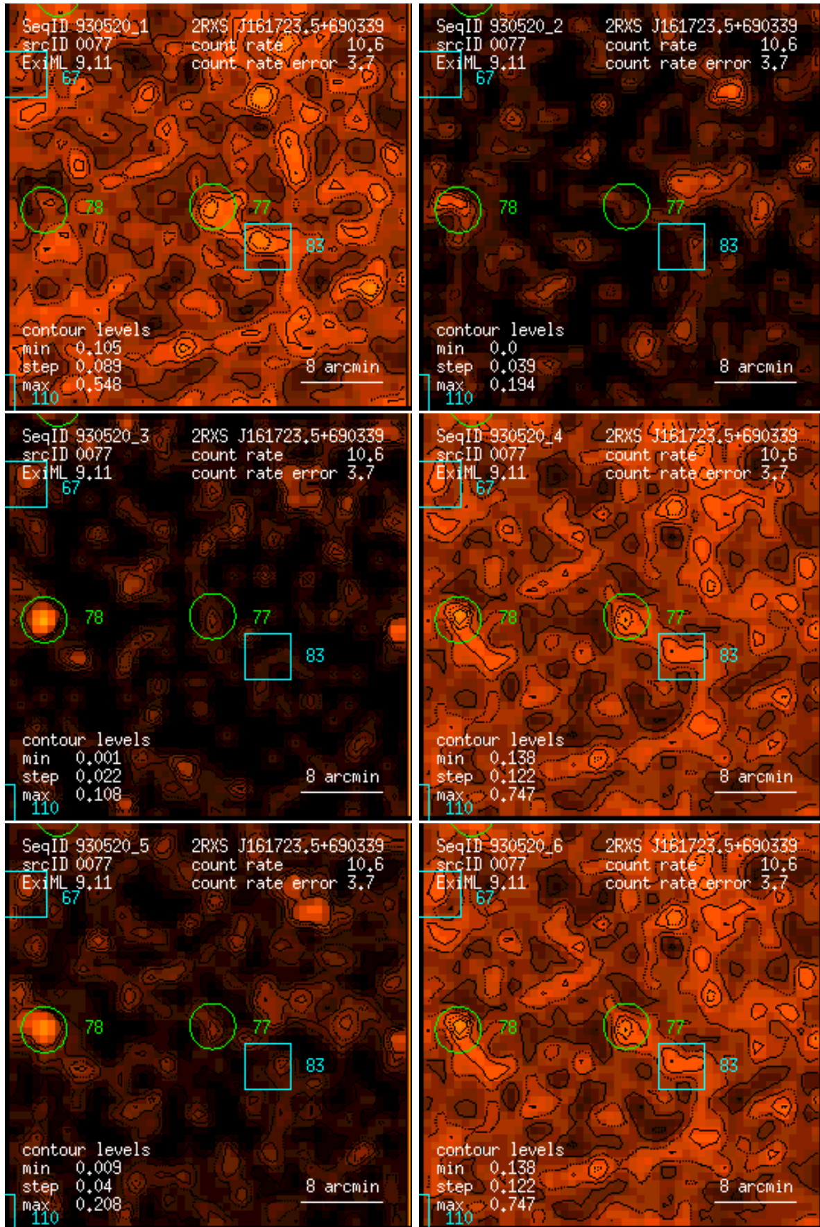
Figure 77: RASS 930520: detection 0077: band rate images, Gaussian filter: (1) PSPC channels 11 – 41, (2) 52 – 90, (3) 91 – 201, (4) 11 – 235, (5) 52 – 201, (6) 11 – 201. Broad band rates in counts/ks. Band rate contour levels in counts/ks/arcmin 2 .
