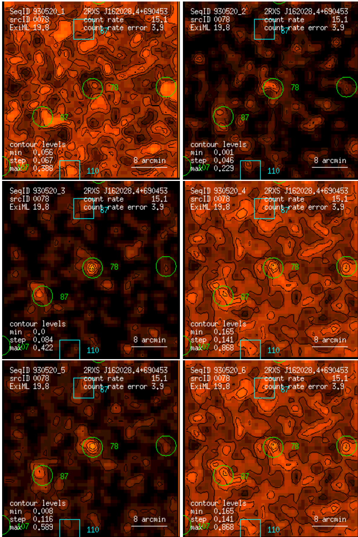
Figure 78: RASS 930520: detection 0078: band rate images, Gaussian filter: (1) PSPC channels 11 – 41, (2) 52 – 90, (3) 91 – 201, (4) 11 – 235, (5) 52 – 201, (6) 11 – 201. Broad band rates in counts/ks. Band rate contour levels in counts/ks/arcmin 2 .
