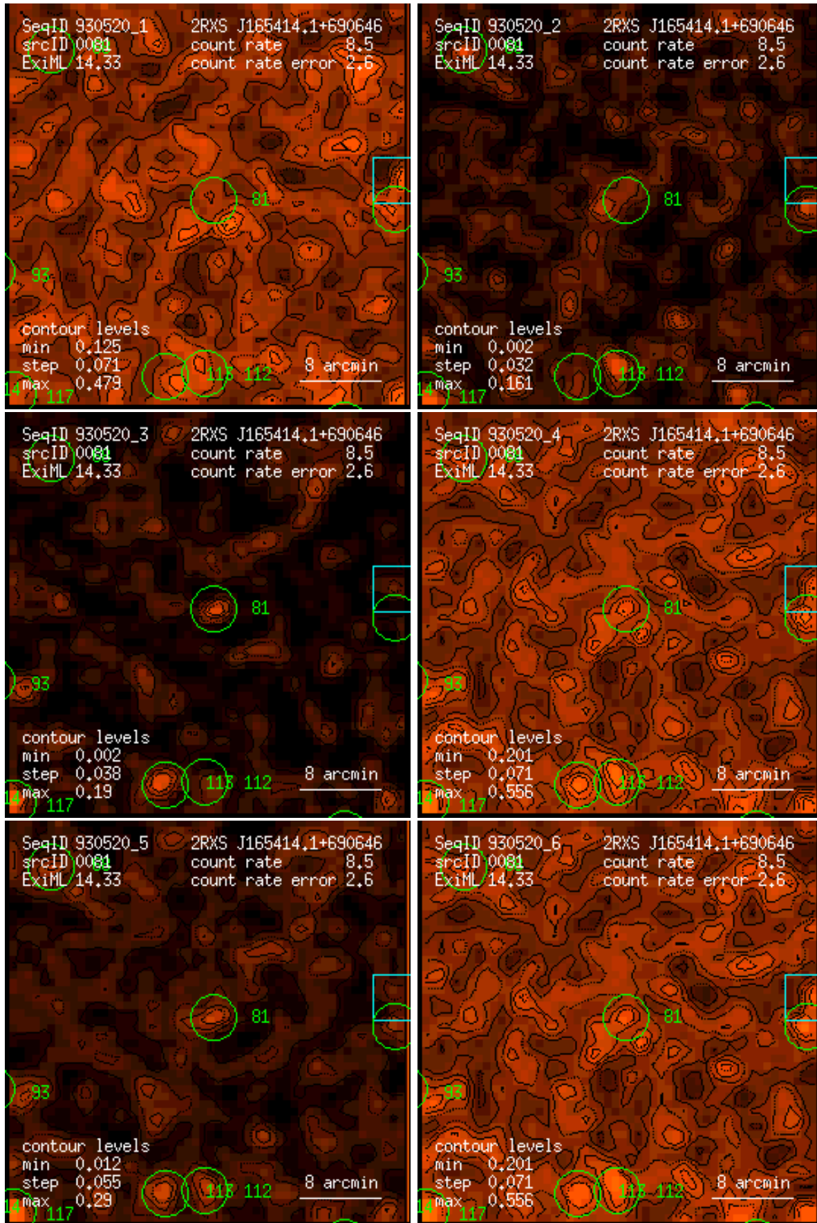
Figure 81: RASS 930520: detection 0081: band rate images, Gaussian filter: (1) PSPC channels 11 – 41, (2) 52 – 90, (3) 91 – 201, (4) 11 – 235, (5) 52 – 201, (6) 11 – 201. Broad band rates in counts/ks. Band rate contour levels in counts/ks/arcmin 2 .
