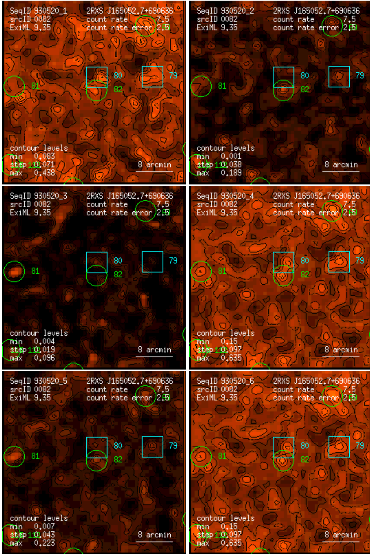
Figure 82: RASS 930520: detection 0082: band rate images, Gaussian filter: (1) PSPC channels 11 – 41, (2) 52 – 90, (3) 91 – 201, (4) 11 – 235, (5) 52 – 201, (6) 11 – 201. Broad band rates in counts/ks. Band rate contour levels in counts/ks/arcmin 2 .
