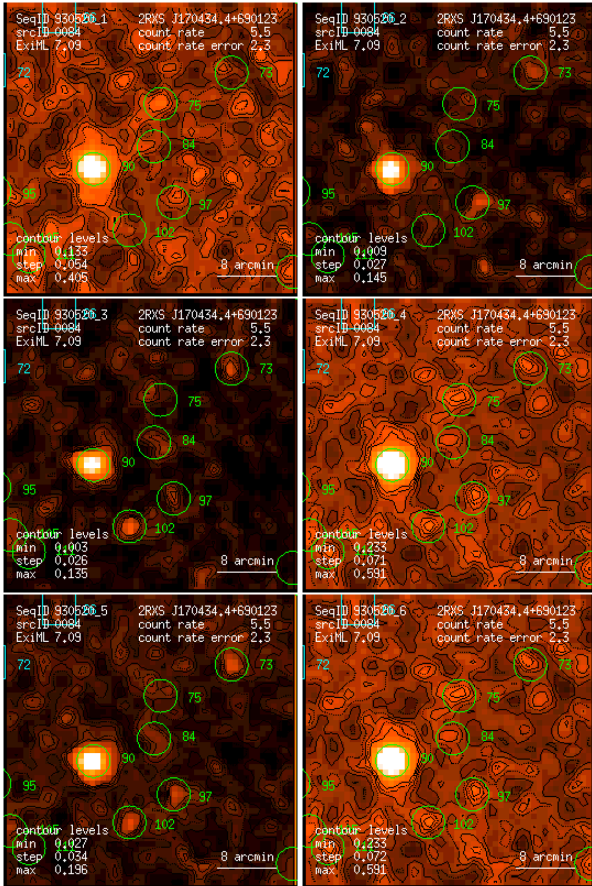
Figure 84: RASS 930520: detection 0084: band rate images, Gaussian filter: (1) PSPC channels 11 – 41, (2) 52 – 90, (3) 91 – 201, (4) 11 – 235, (5) 52 – 201, (6) 11 – 201. Broad band rates in counts/ks. Band rate contour levels in counts/ks/arcmin 2 .
