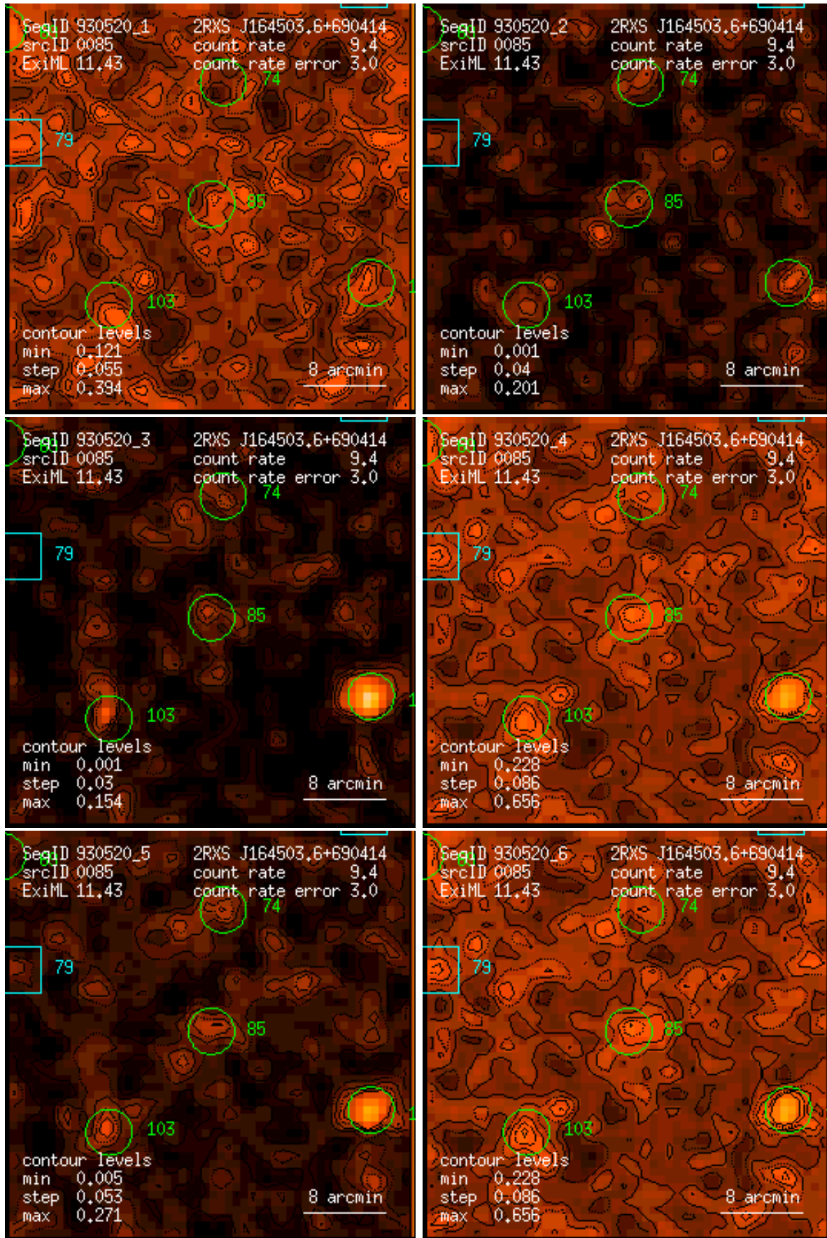
Figure 85: RASS 930520: detection 0085: band rate images, Gaussian filter: (1) PSPC channels 11 – 41, (2) 52 – 90, (3) 91 – 201, (4) 11 – 235, (5) 52 – 201, (6) 11 – 201. Broad band rates in counts/ks. Band rate contour levels in counts/ks/arcmin 2 .
