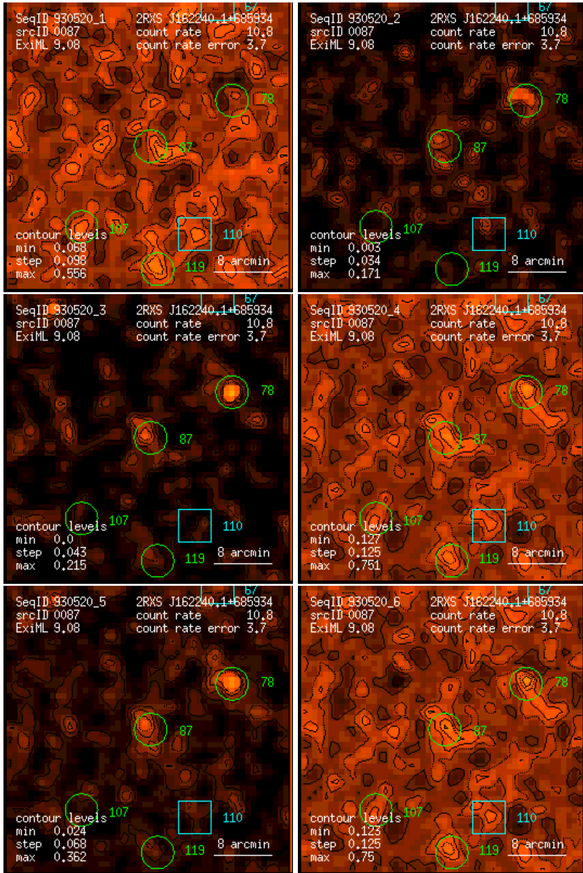
Figure 87: RASS 930520: detection 0087: band rate images, Gaussian filter: (1) PSPC channels 11 – 41, (2) 52 – 90, (3) 91 – 201, (4) 11 – 235, (5) 52 – 201, (6) 11 – 201. Broad band rates in counts/ks. Band rate contour levels in counts/ks/arcmin 2 .
