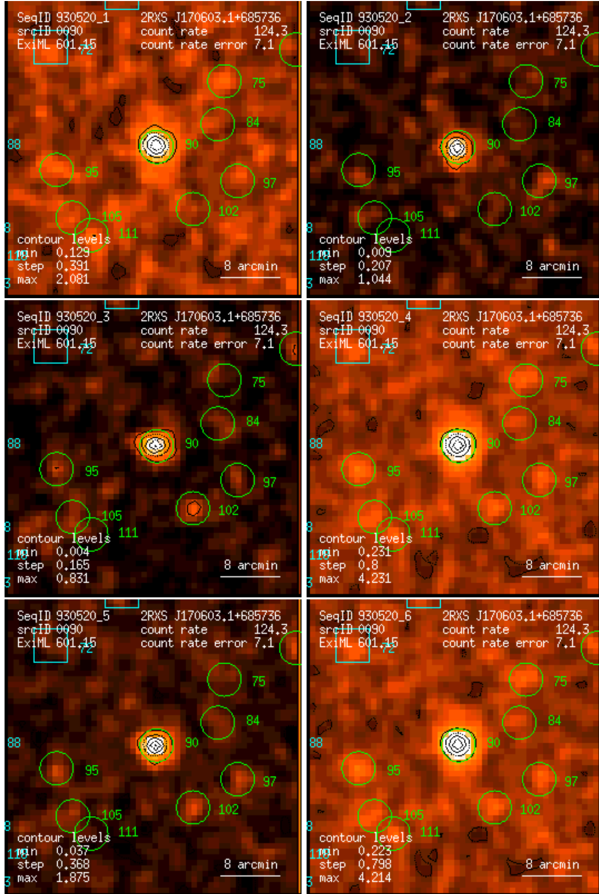
Figure 90: RASS 930520: detection 0090: band rate images, Gaussian filter: (1) PSPC channels 11 – 41, (2) 52 – 90, (3) 91 – 201, (4) 11 – 235, (5) 52 – 201, (6) 11 – 201. Broad band rates in counts/ks. Band rate contour levels in counts/ks/arcmin 2 .
