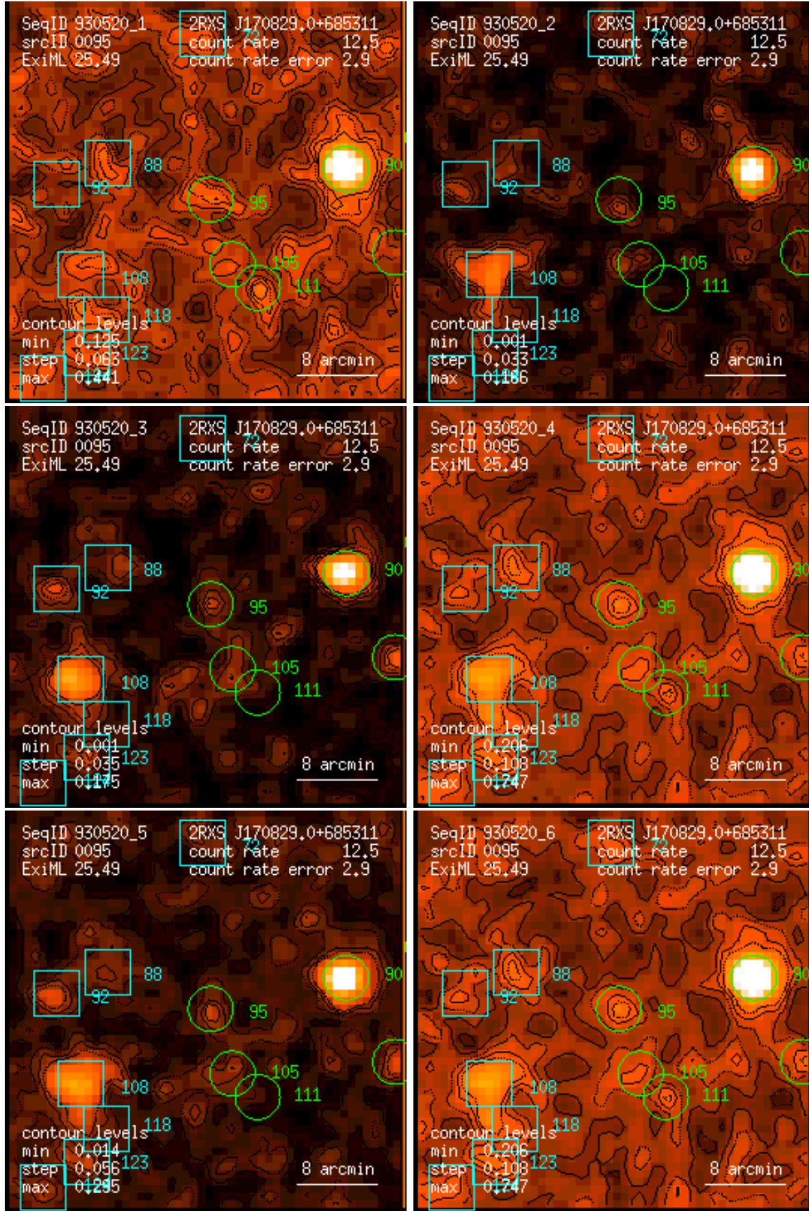
Figure 95: RASS 930520: detection 0095: band rate images, Gaussian filter: (1) PSPC channels 11 – 41, (2) 52 – 90, (3) 91 – 201, (4) 11 – 235, (5) 52 – 201, (6) 11 – 201. Broad band rates in counts/ks. Band rate contour levels in counts/ks/arcmin 2 .
