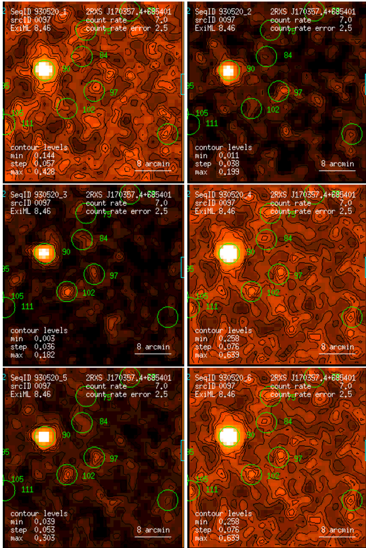
Figure 97: RASS 930520: detection 0097: band rate images, Gaussian filter: (1) PSPC channels 11 – 41, (2) 52 – 90, (3) 91 – 201, (4) 11 – 235, (5) 52 – 201, (6) 11 – 201. Broad band rates in counts/ks. Band rate contour levels in counts/ks/arcmin 2 .
