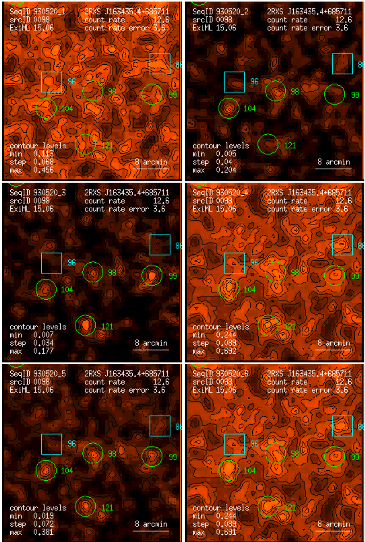
Figure 98: RASS 930520: detection 0098: band rate images, Gaussian filter: (1) PSPC channels 11 – 41, (2) 52 – 90, (3) 91 – 201, (4) 11 – 235, (5) 52 – 201, (6) 11 – 201. Broad band rates in counts/ks. Band rate contour levels in counts/ks/arcmin 2 .
