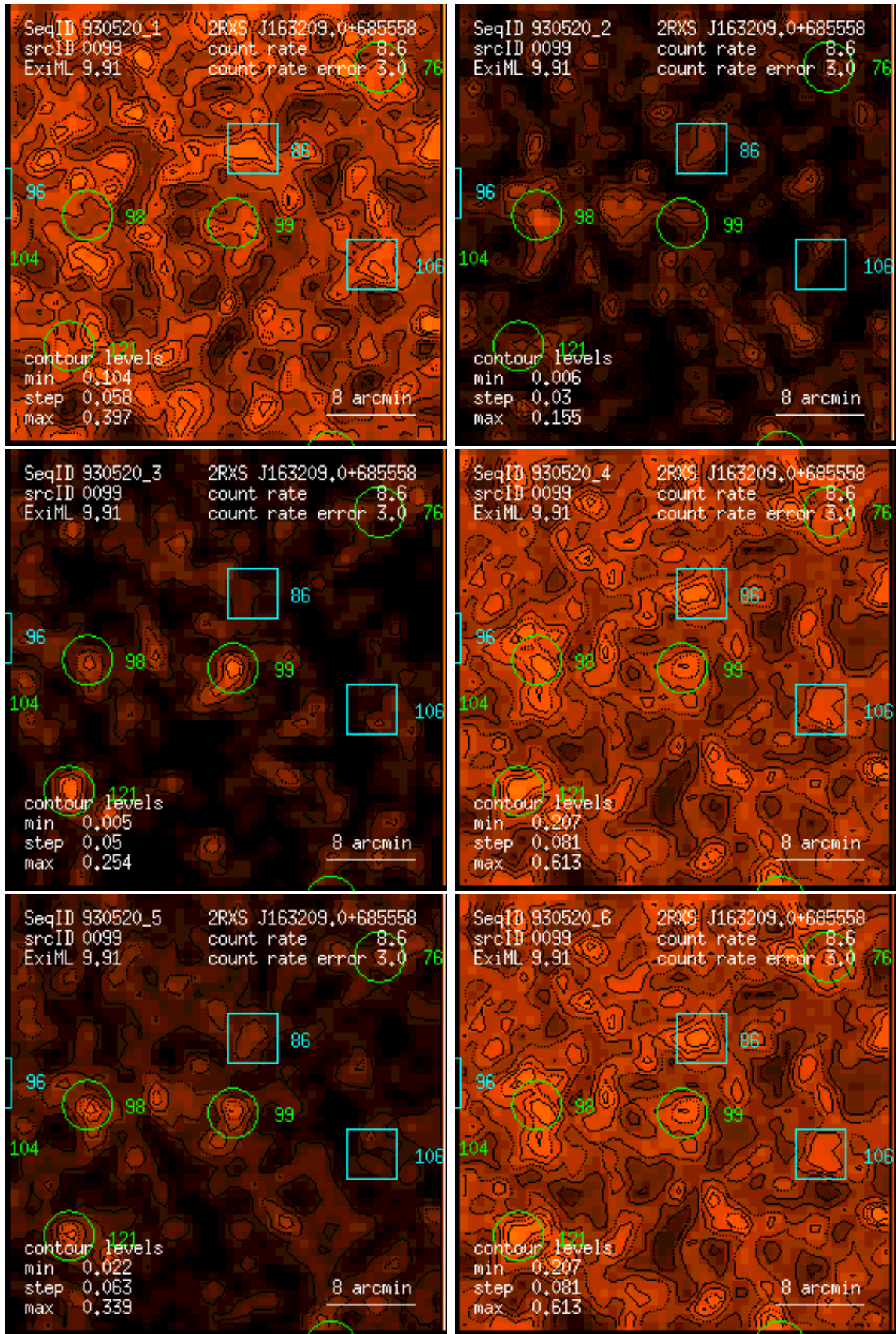
Figure 99: RASS 930520: detection 0099: band rate images, Gaussian filter: (1) PSPC channels 11 – 41, (2) 52 – 90, (3) 91 – 201, (4) 11 – 235, (5) 52 – 201, (6) 11 – 201. Broad band rates in counts/ks. Band rate contour levels in counts/ks/arcmin 2 .
