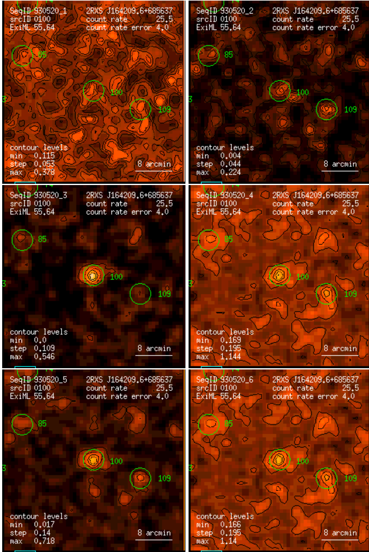
Figure 100: RASS 930520: detection 0100: band rate images, Gaussian filter: (1) PSPC channels 11 – 41, (2) 52 – 90, (3) 91 – 201, (4) 11 – 235, (5) 52 – 201, (6) 11 – 201. Broad band rates in counts/ks. Band rate contour levels in counts/ks/arcmin 2 .
