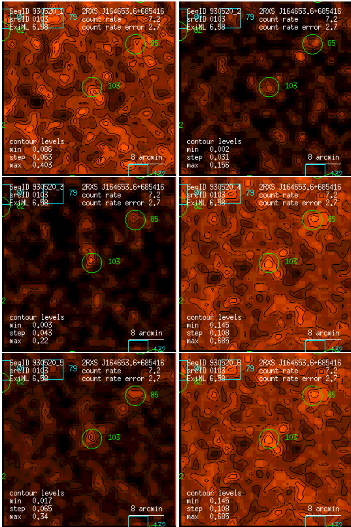
Figure 103: RASS 930520: detection 0103: band rate images, Gaussian filter: (1) PSPC channels 11 – 41, (2) 52 – 90, (3) 91 – 201, (4) 11 – 235, (5) 52 – 201, (6) 11 – 201. Broad band rates in counts/ks. Band rate contour levels in counts/ks/arcmin 2 .
