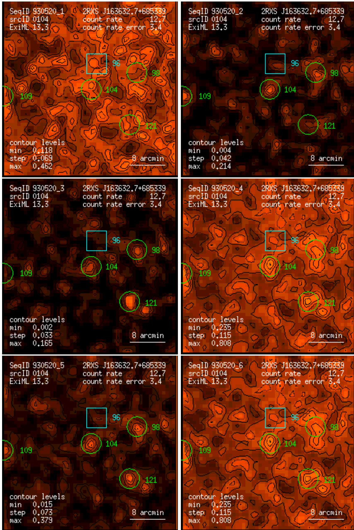
Figure 104: RASS 930520: detection 0104: band rate images, Gaussian filter: (1) PSPC channels 11 – 41, (2) 52 – 90, (3) 91 – 201, (4) 11 – 235, (5) 52 – 201, (6) 11 – 201. Broad band rates in counts/ks. Band rate contour levels in counts/ks/arcmin 2 .
