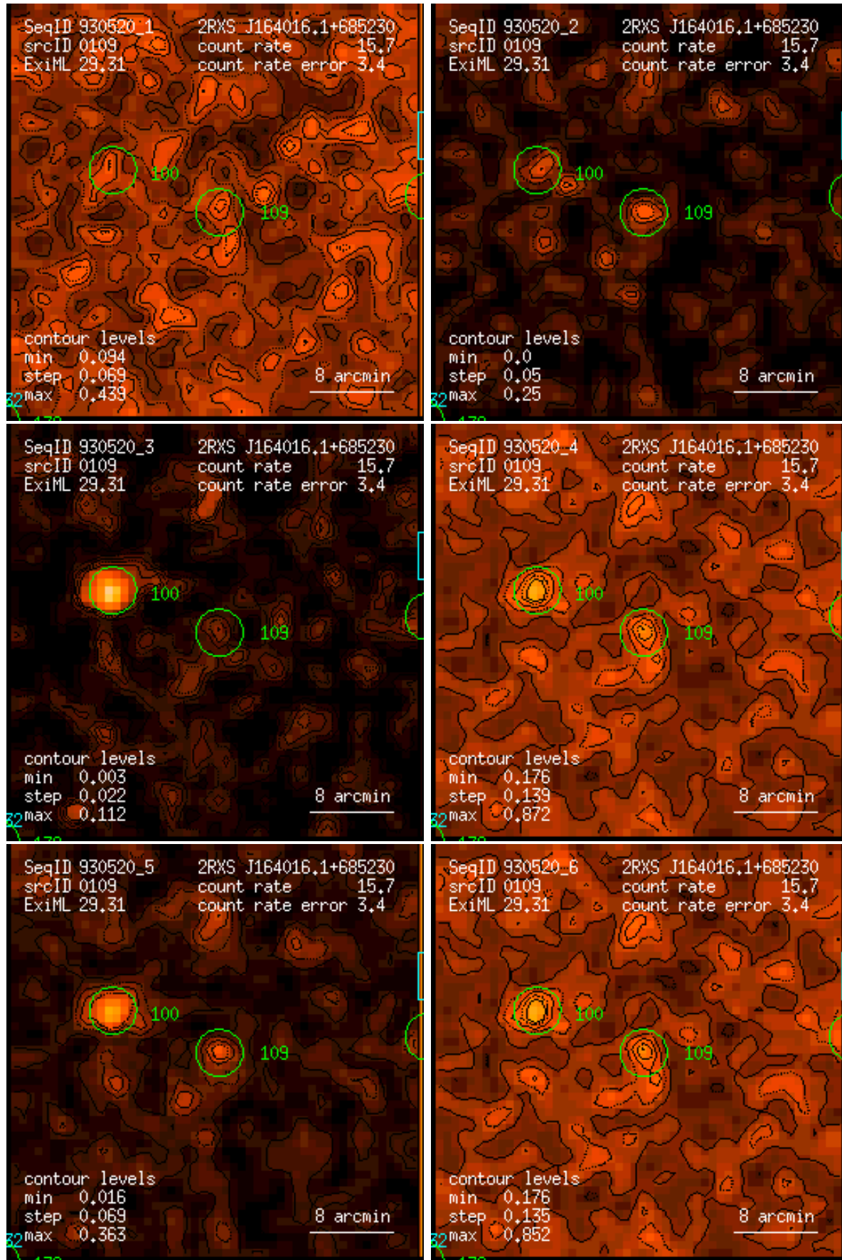
Figure 109: RASS 930520: detection 0109: band rate images, Gaussian filter: (1) PSPC channels 11 – 41, (2) 52 – 90, (3) 91 – 201, (4) 11 – 235, (5) 52 – 201, (6) 11 – 201. Broad band rates in counts/ks. Band rate contour levels in counts/ks/arcmin 2 .
