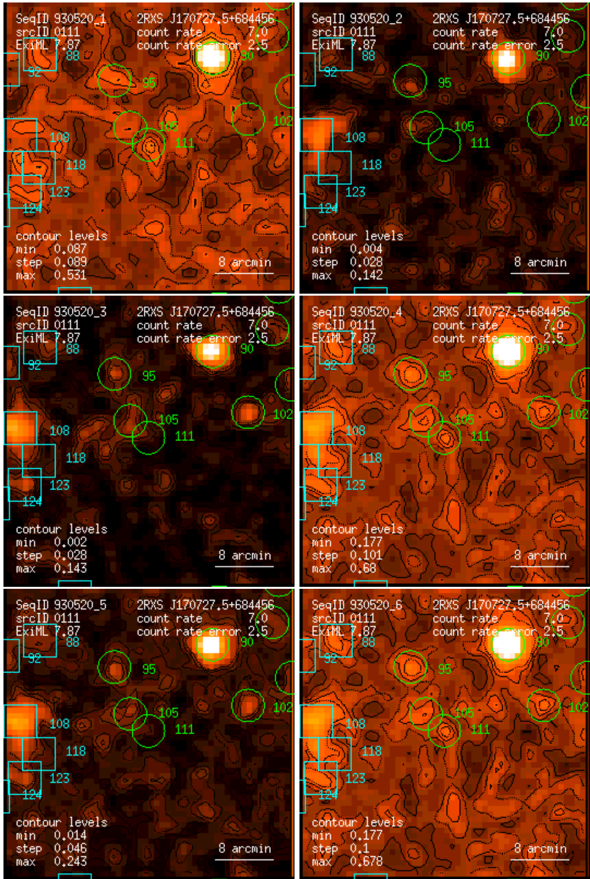
Figure 111: RASS 930520: detection 0111: band rate images, Gaussian filter: (1) PSPC channels 11 – 41, (2) 52 – 90, (3) 91 – 201, (4) 11 – 235, (5) 52 – 201, (6) 11 – 201. Broad band rates in counts/ks. Band rate contour levels in counts/ks/arcmin 2 .
