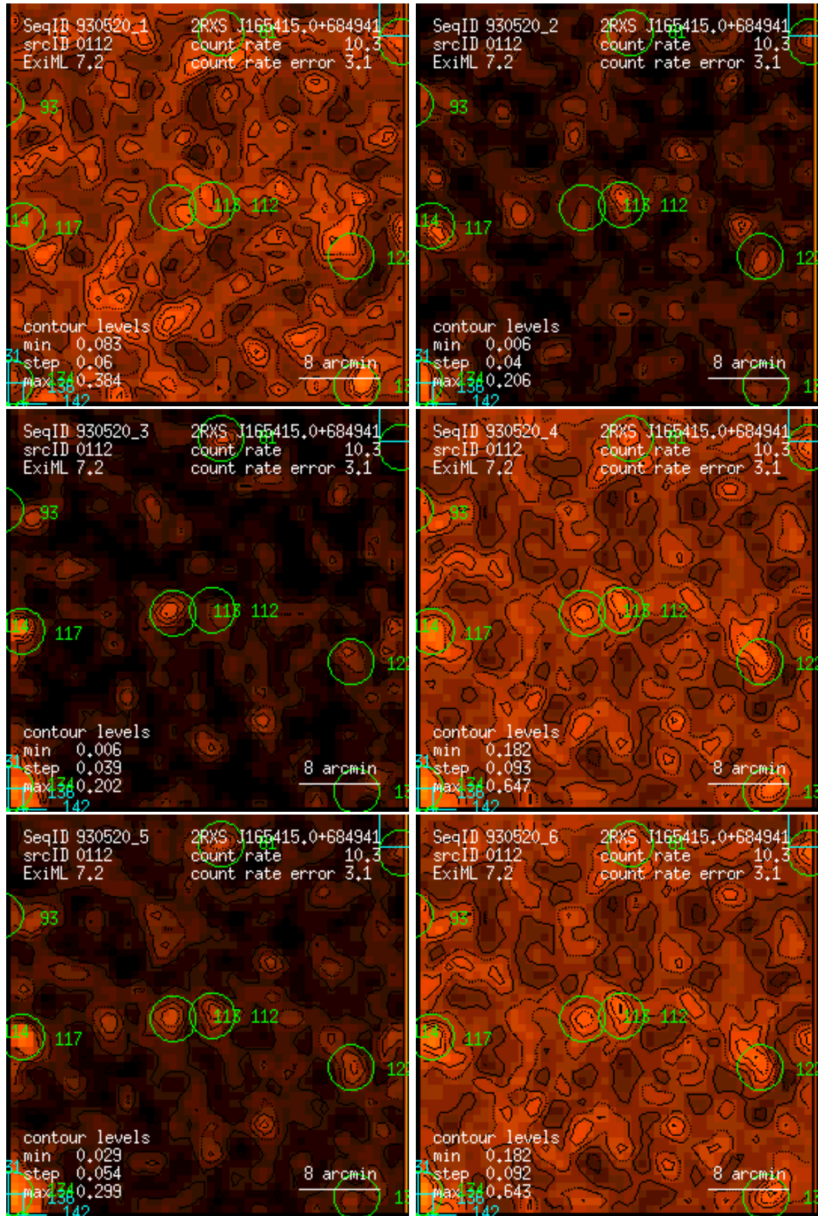
Figure 112: RASS 930520: detection 0112: band rate images, Gaussian filter: (1) PSPC channels 11 – 41, (2) 52 – 90, (3) 91 – 201, (4) 11 – 235, (5) 52 – 201, (6) 11 – 201. Broad band rates in counts/ks. Band rate contour levels in counts/ks/arcmin 2 .
