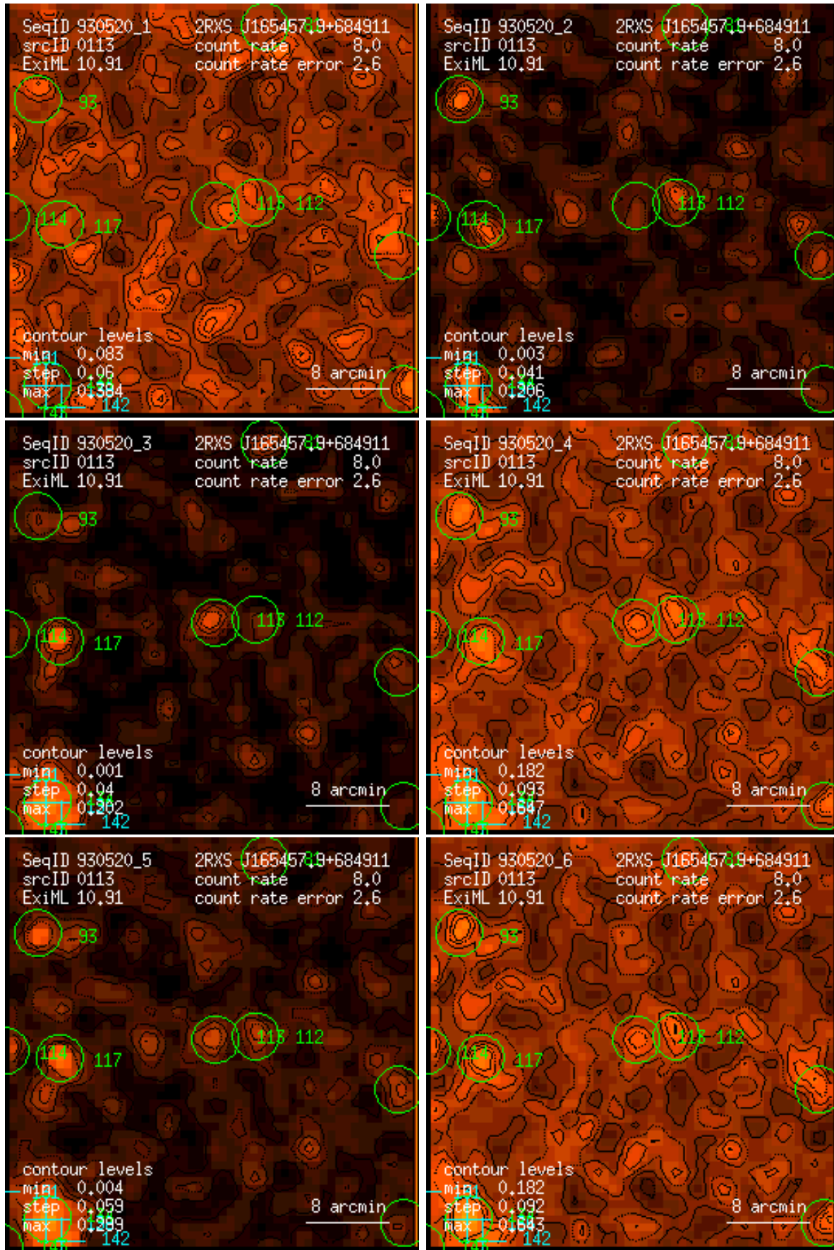
Figure 113: RASS 930520: detection 0113: band rate images, Gaussian filter: (1) PSPC channels 11 – 41, (2) 52 – 90, (3) 91 – 201, (4) 11 – 235, (5) 52 – 201, (6) 11 – 201. Broad band rates in counts/ks. Band rate contour levels in counts/ks/arcmin 2 .
