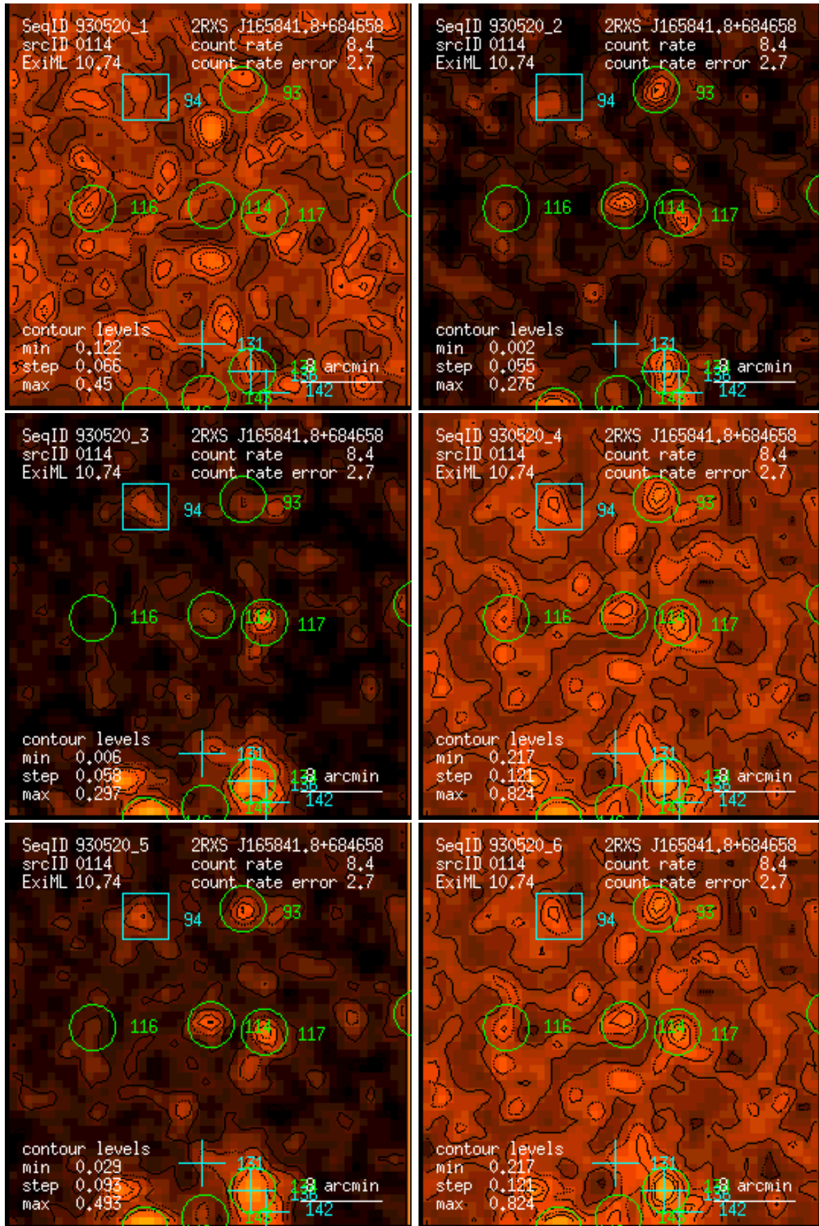
Figure 114: RASS 930520: detection 0114: band rate images, Gaussian filter: (1) PSPC channels 11 – 41, (2) 52 – 90, (3) 91 – 201, (4) 11 – 235, (5) 52 – 201, (6) 11 – 201. Broad band rates in counts/ks. Band rate contour levels in counts/ks/arcmin 2 .
