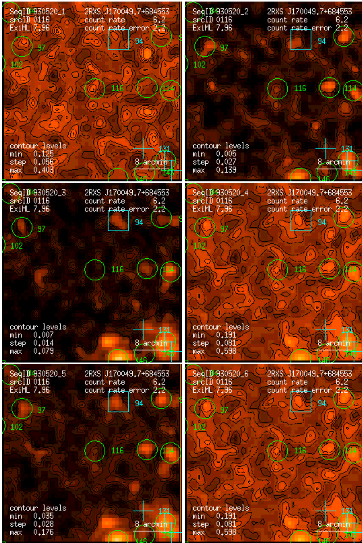
Figure 116: RASS 930520: detection 0116: band rate images, Gaussian filter: (1) PSPC channels 11 – 41, (2) 52 – 90, (3) 91 – 201, (4) 11 – 235, (5) 52 – 201, (6) 11 – 201. Broad band rates in counts/ks. Band rate contour levels in counts/ks/arcmin 2 .
