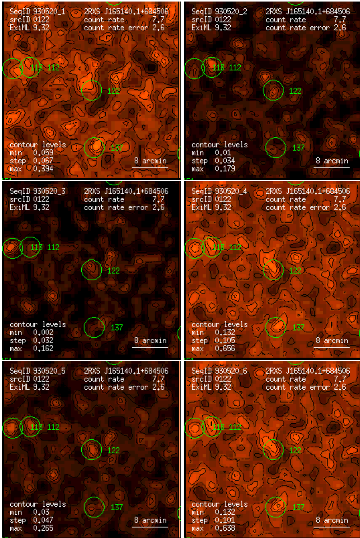
Figure 122: RASS 930520: detection 0122: band rate images, Gaussian filter: (1) PSPC channels 11 – 41, (2) 52 – 90, (3) 91 – 201, (4) 11 – 235, (5) 52 – 201, (6) 11 – 201. Broad band rates in counts/ks. Band rate contour levels in counts/ks/arcmin 2 .
