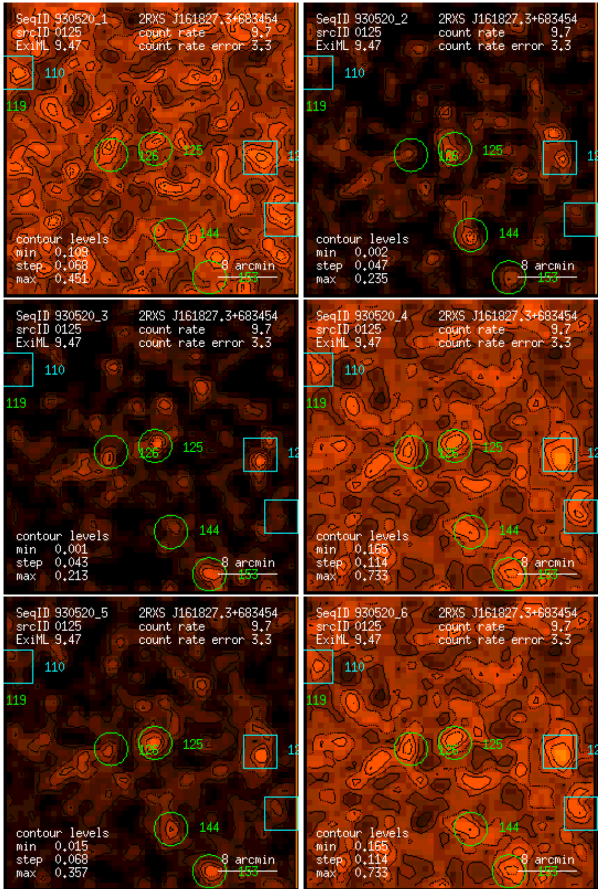
Figure 125: RASS 930520: detection 0125: band rate images, Gaussian filter: (1) PSPC channels 11 – 41, (2) 52 – 90, (3) 91 – 201, (4) 11 – 235, (5) 52 – 201, (6) 11 – 201. Broad band rates in counts/ks. Band rate contour levels in counts/ks/arcmin 2 .
