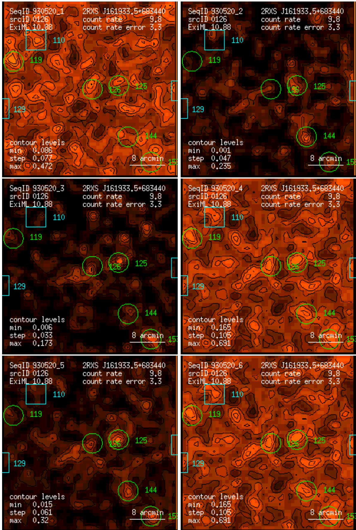
Figure 126: RASS 930520: detection 0126: band rate images, Gaussian filter: (1) PSPC channels 11 – 41, (2) 52 – 90, (3) 91 – 201, (4) 11 – 235, (5) 52 – 201, (6) 11 – 201. Broad band rates in counts/ks. Band rate contour levels in counts/ks/arcmin 2 .
