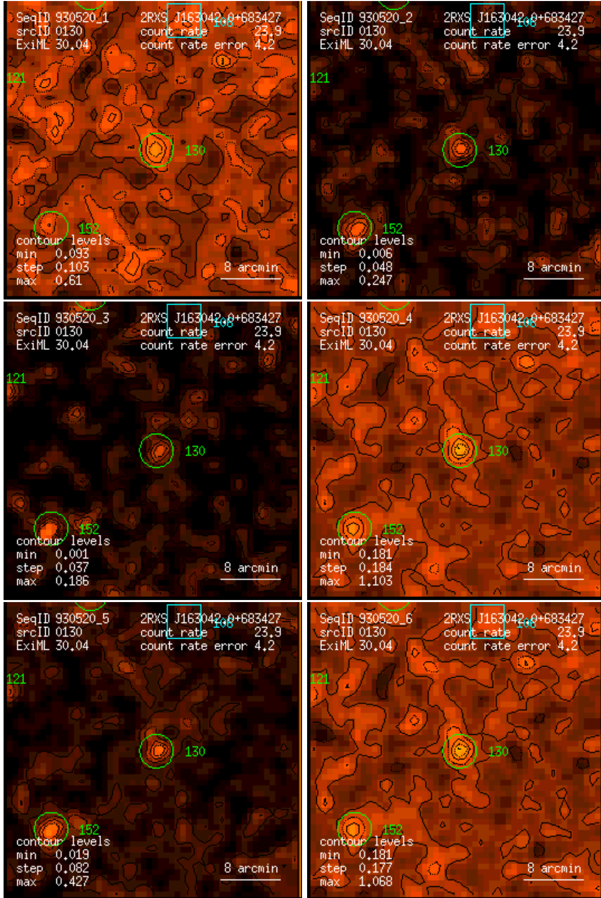
Figure 130: RASS 930520: detection 0130: band rate images, Gaussian filter: (1) PSPC channels 11 – 41, (2) 52 – 90, (3) 91 – 201, (4) 11 – 235, (5) 52 – 201, (6) 11 – 201. Broad band rates in counts/ks. Band rate contour levels in counts/ks/arcmin 2 .
