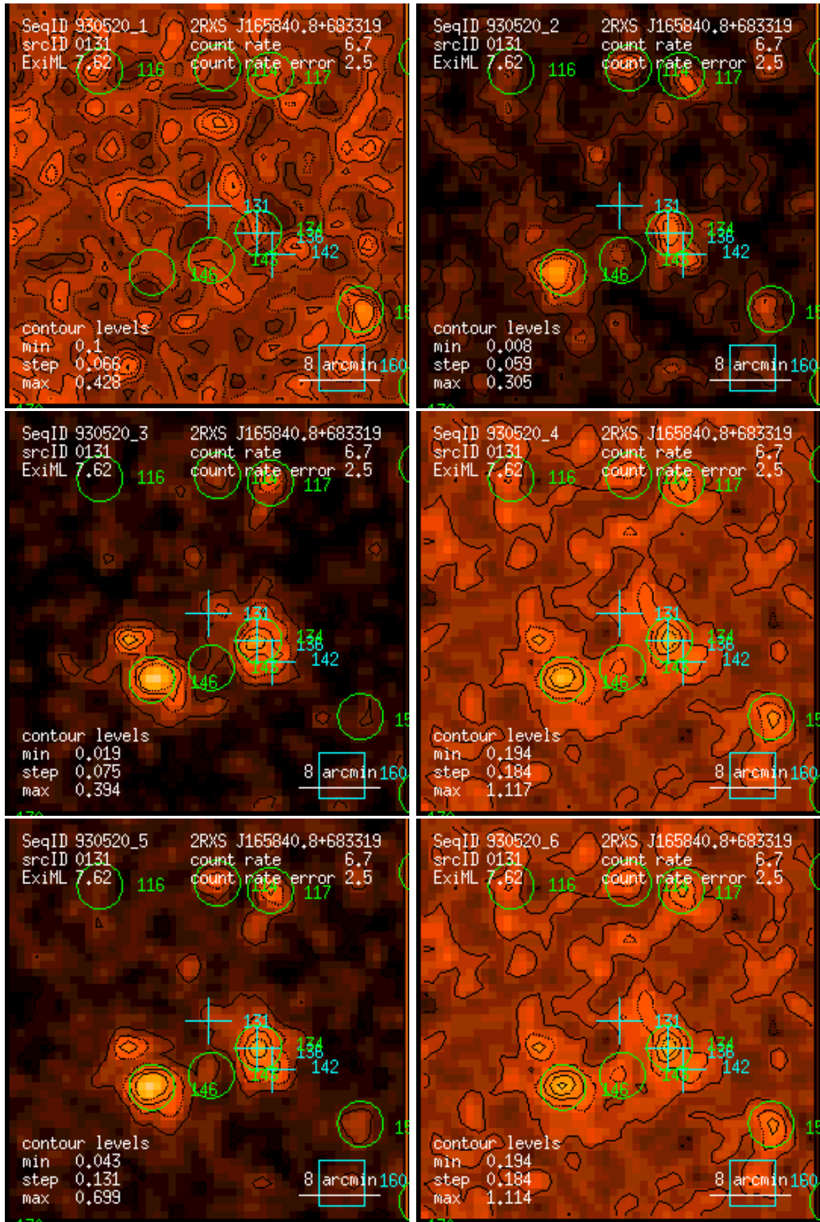
Figure 131: RASS 930520: detection 0131: band rate images, Gaussian filter: (1) PSPC channels 11 – 41, (2) 52 – 90, (3) 91 – 201, (4) 11 – 235, (5) 52 – 201, (6) 11 – 201. Broad band rates in counts/ks. Band rate contour levels in counts/ks/arcmin 2 .
