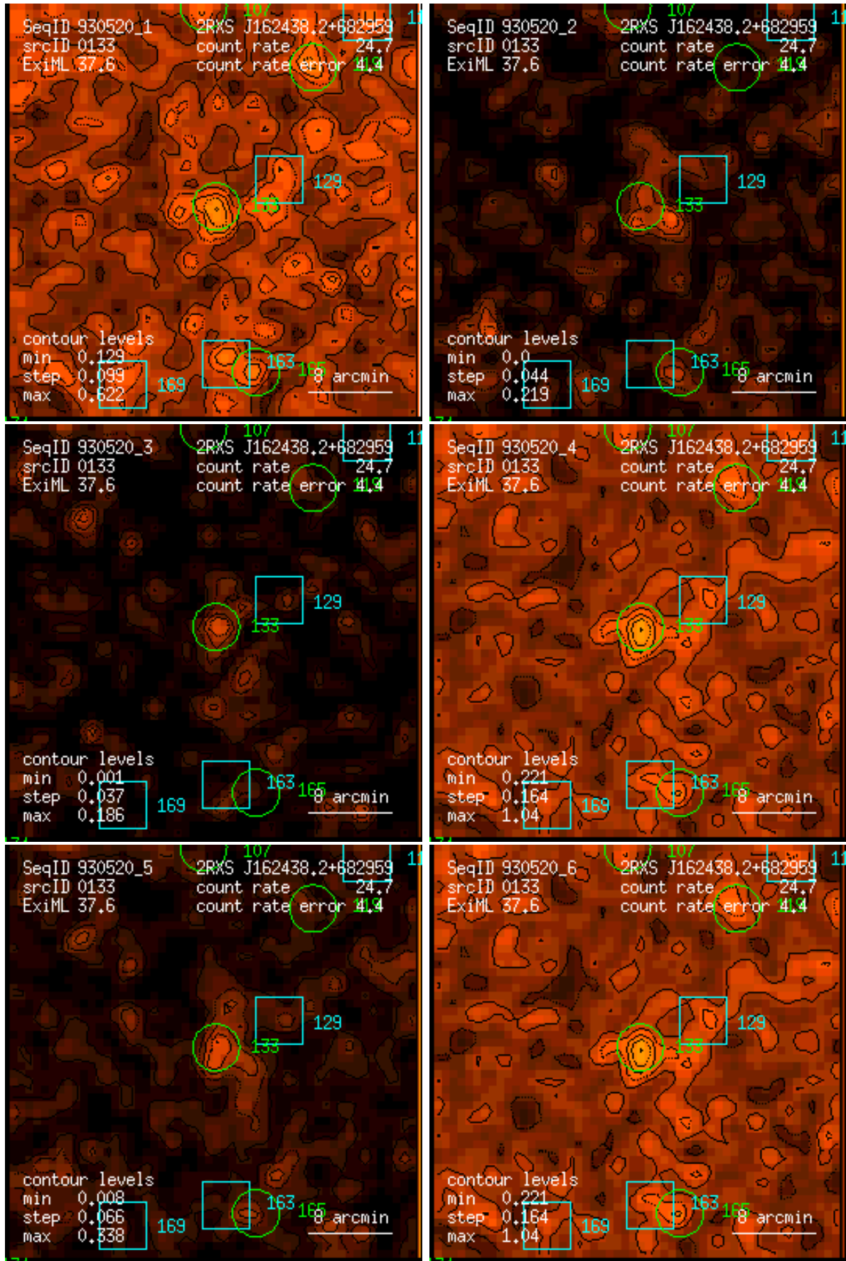
Figure 133: RASS 930520: detection 0133: band rate images, Gaussian filter: (1) PSPC channels 11 – 41, (2) 52 – 90, (3) 91 – 201, (4) 11 – 235, (5) 52 – 201, (6) 11 – 201. Broad band rates in counts/ks. Band rate contour levels in counts/ks/arcmin 2 .
