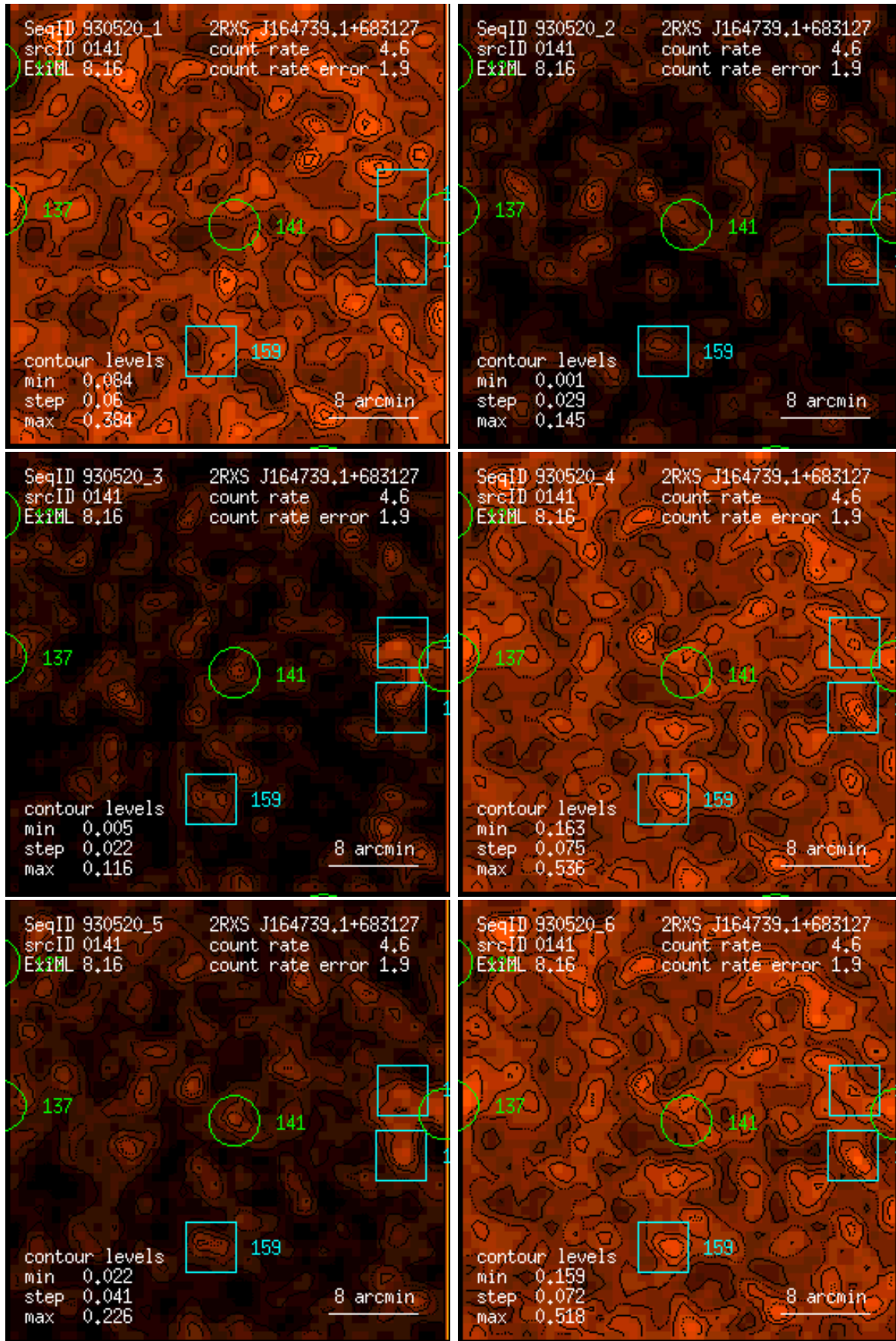
Figure 141: RASS 930520: detection 0141: band rate images, Gaussian filter: (1) PSPC channels 11 – 41, (2) 52 – 90, (3) 91 – 201, (4) 11 – 235, (5) 52 – 201, (6) 11 – 201. Broad band rates in counts/ks. Band rate contour levels in counts/ks/arcmin 2 .
