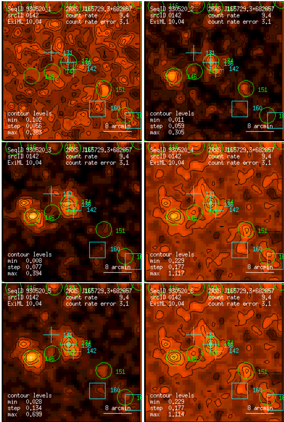
Figure 142: RASS 930520: detection 0142: band rate images, Gaussian filter: (1) PSPC channels 11 – 41, (2) 52 – 90, (3) 91 – 201, (4) 11 – 235, (5) 52 – 201, (6) 11 – 201. Broad band rates in counts/ks. Band rate contour levels in counts/ks/arcmin 2 .
