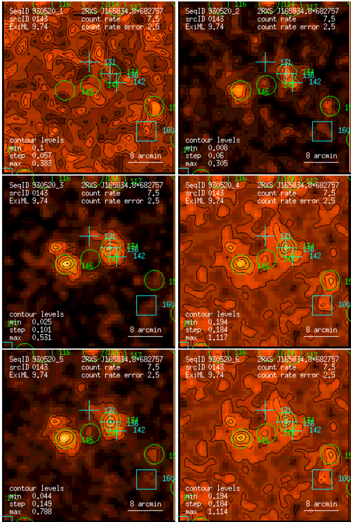
Figure 143: RASS 930520: detection 0143: band rate images, Gaussian filter: (1) PSPC channels 11 – 41, (2) 52 – 90, (3) 91 – 201, (4) 11 – 235, (5) 52 – 201, (6) 11 – 201. Broad band rates in counts/ks. Band rate contour levels in counts/ks/arcmin 2 .
