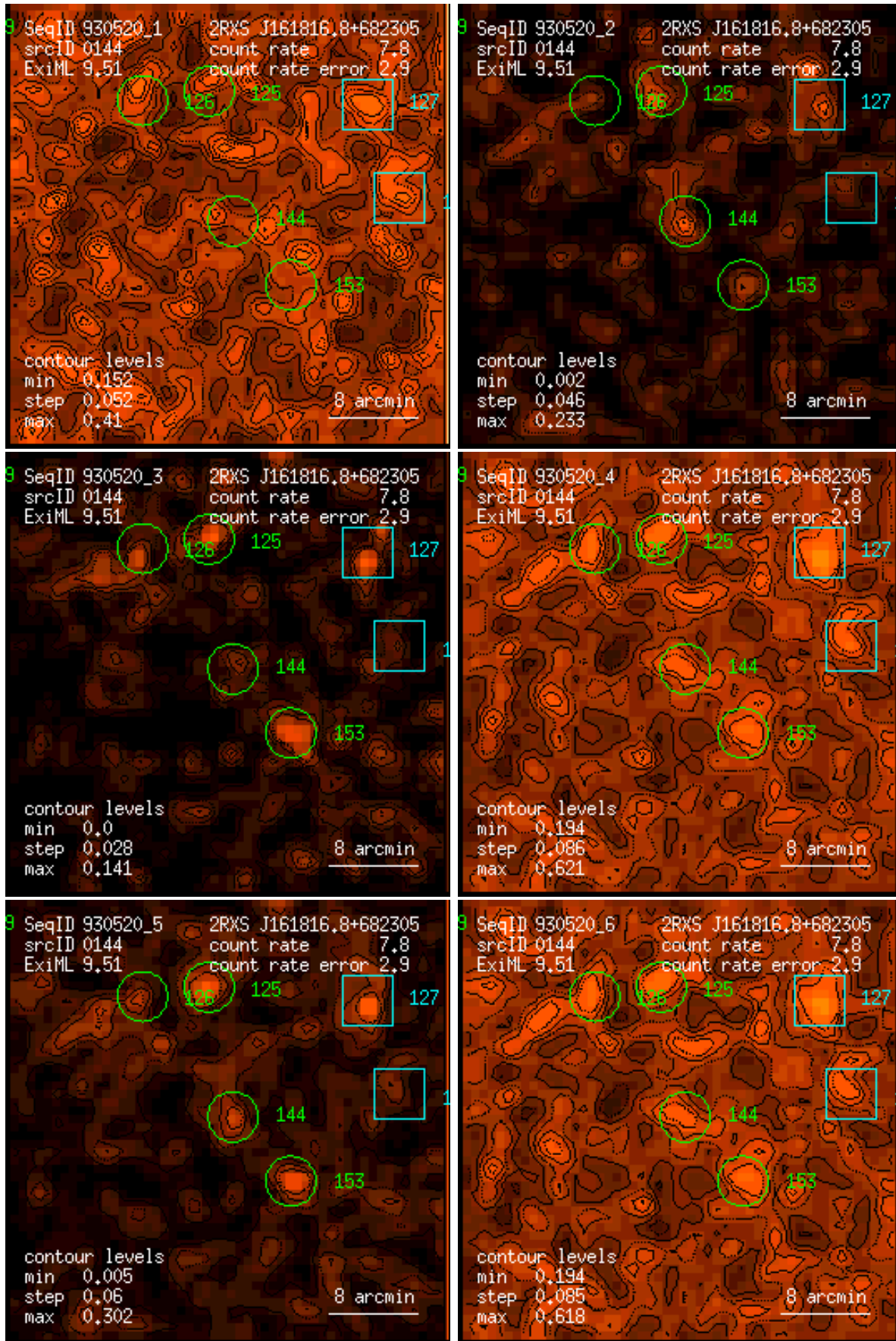
Figure 144: RASS 930520: detection 0144: band rate images, Gaussian filter: (1) PSPC channels 11 – 41, (2) 52 – 90, (3) 91 – 201, (4) 11 – 235, (5) 52 – 201, (6) 11 – 201. Broad band rates in counts/ks. Band rate contour levels in counts/ks/arcmin 2 .
