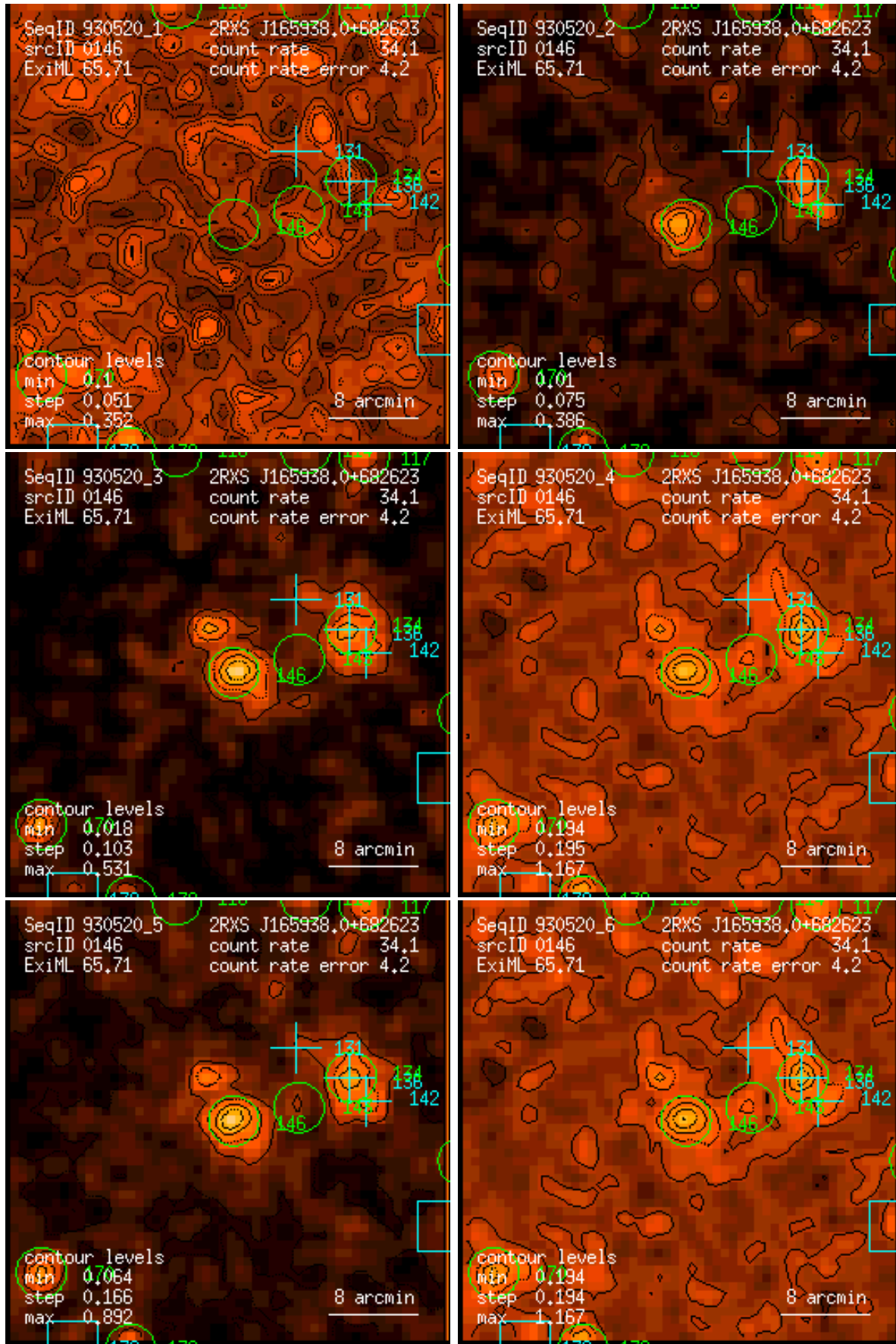
Figure 146: RASS 930520: detection 0146: band rate images, Gaussian filter: (1) PSPC channels 11 – 41, (2) 52 – 90, (3) 91 – 201, (4) 11 – 235, (5) 52 – 201, (6) 11 – 201. Broad band rates in counts/ks. Band rate contour levels in counts/ks/arcmin 2 .
