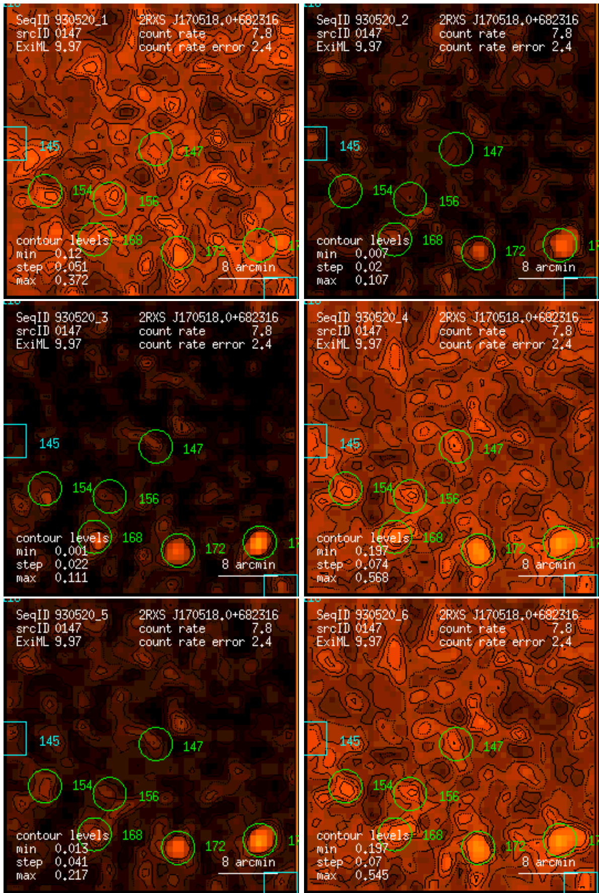
Figure 147: RASS 930520: detection 0147: band rate images, Gaussian filter: (1) PSPC channels 11 – 41, (2) 52 – 90, (3) 91 – 201, (4) 11 – 235, (5) 52 – 201, (6) 11 – 201. Broad band rates in counts/ks. Band rate contour levels in counts/ks/arcmin 2 .
