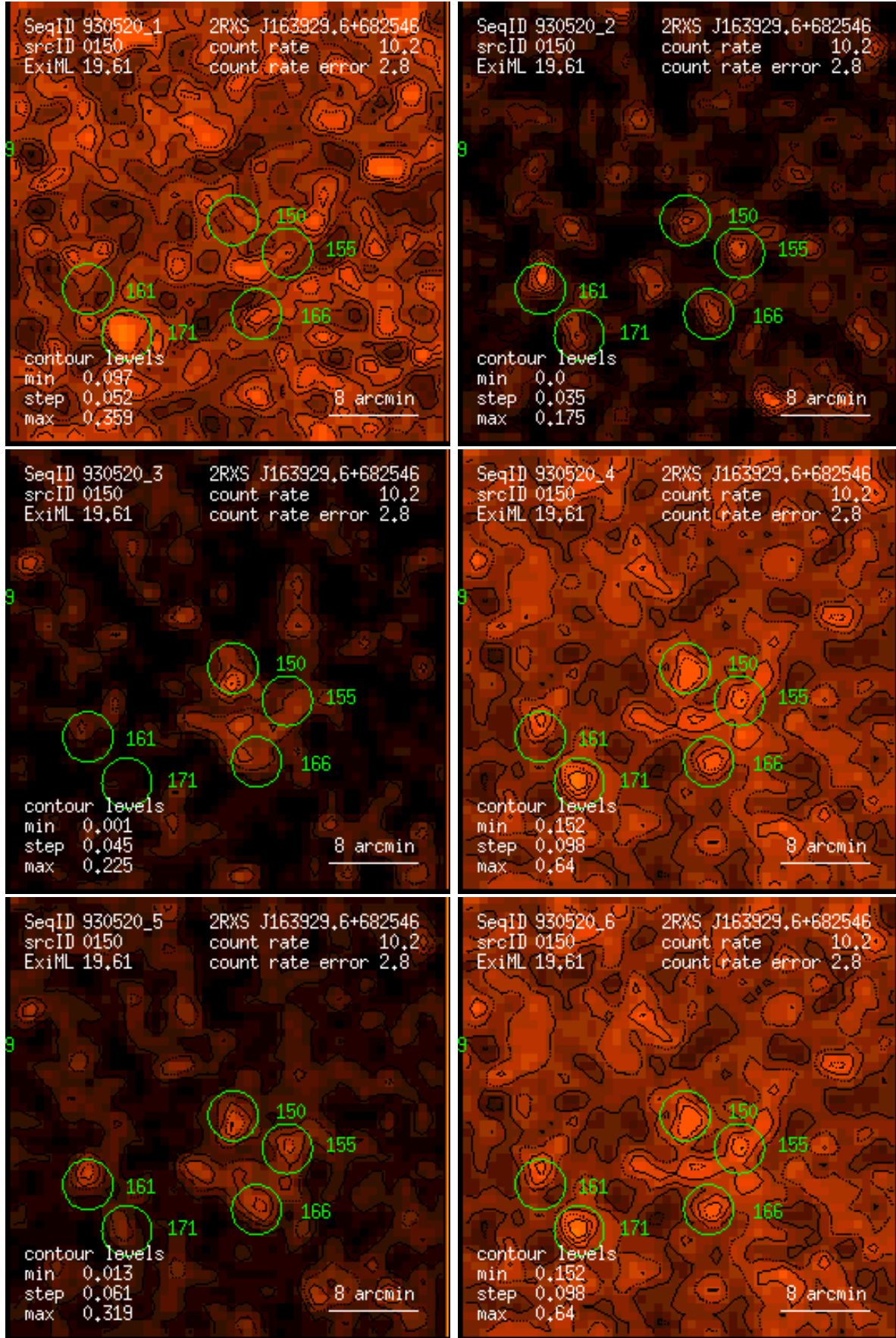
Figure 150: RASS 930520: detection 0150: band rate images, Gaussian filter: (1) PSPC channels 11 – 41, (2) 52 – 90, (3) 91 – 201, (4) 11 – 235, (5) 52 – 201, (6) 11 – 201. Broad band rates in counts/ks. Band rate contour levels in counts/ks/arcmin 2 .
