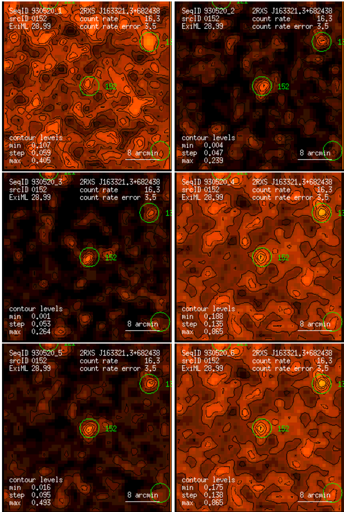
Figure 152: RASS 930520: detection 0152: band rate images, Gaussian filter: (1) PSPC channels 11 – 41, (2) 52 – 90, (3) 91 – 201, (4) 11 – 235, (5) 52 – 201, (6) 11 – 201. Broad band rates in counts/ks. Band rate contour levels in counts/ks/arcmin 2 .
